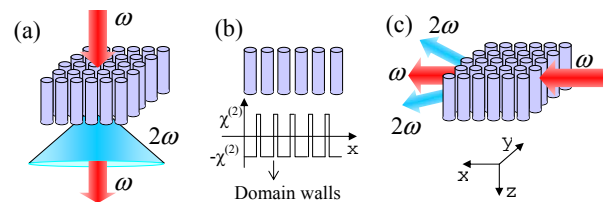
Fig. 1. (color online) (a) Čerenkov SHG with fundamental beam propagating along domain walls. (b) Definition of domain walls. (c) Čerenkov SHG with fundamental beam propagating in the plane of \chi^{(2)} modulation.
