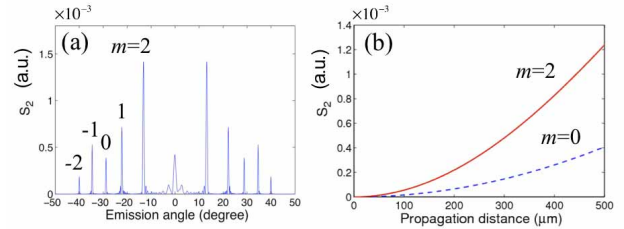
Fig. 4. (color online) (a) Čerenkov SHG at multiple directions; (b) The generated SH signal as a function of propagation distance.
