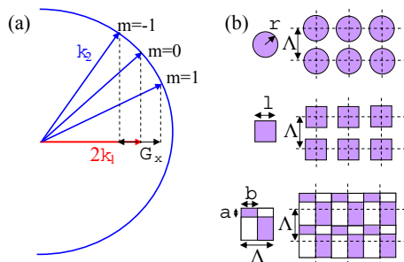
Fig. 2. (color online) (a) Čerenkov SHG with m = 0, \pm 1 . (b) Different shapes of the reversed domains: circular, square and chessboard-like structures.
