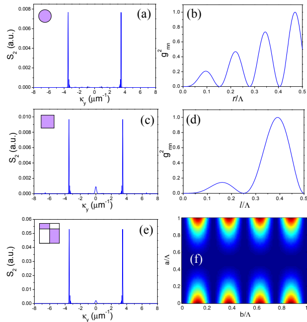
Fig. 3. (color online) Left column: Čerenkov SHG in 2D NPC formed by circular, square and chessboard-like reversed domains. Right column: The effect of duty cycle.
