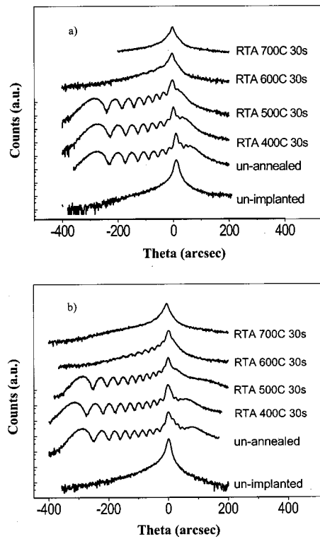
FIG. 1. X-ray rocking curves from InP implanted at 200 °C with a dose of 1 \times 10^{16} \text{ cm}^{-2} . 1 MeV \text{P}^+ (a) and 2 MeV \text{As}^+ (b). Spectra vertically shifted for clarity.
