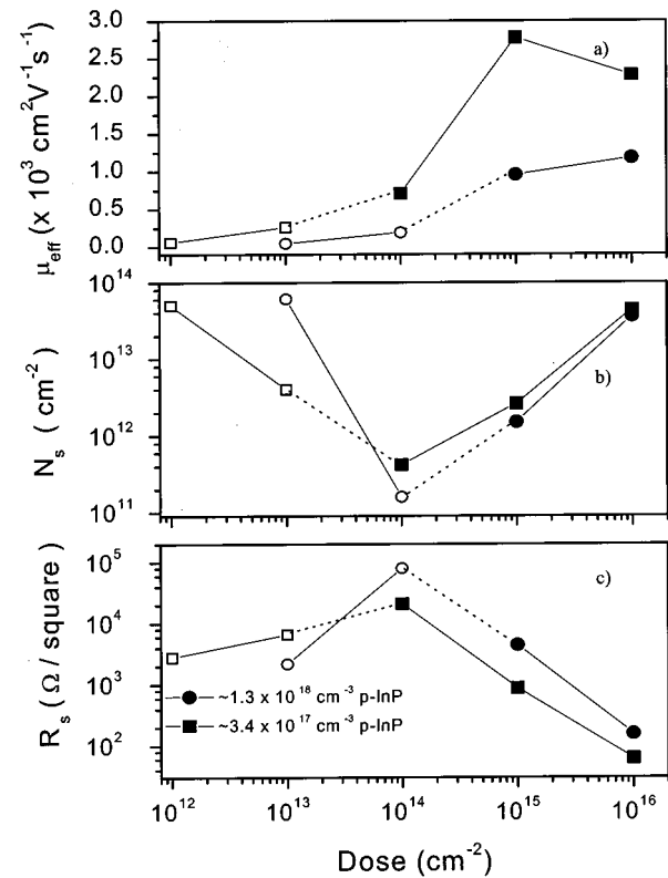
FIG. 4. Mobility (a), sheet carrier concentration (b), and sheet resistance (c) as a function of P^+ implant dose, for p -type InP with hole concentrations \sim 3.4 \times 10^{17} and \sim 1.3 \times 10^{18} cm^{-3} . Samples annealed at 600^\circ C for 30 s. Open symbols signify p type, and closed symbols signify n type. Joining lines are guides for the eye only.
