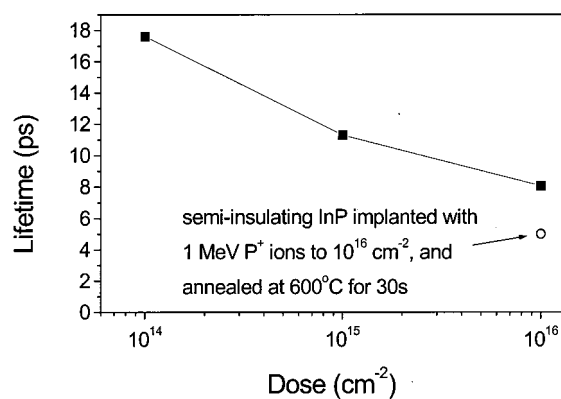
FIG. 5. Plot of time-resolved photoluminescence decay times for p -InP ( \sim 3.4 \times 10^{17} \text{ cm}^{-3} ) implanted with different doses of 1 MeV \text{P}^+ ions at 200 °C, subsequently annealed by RTA 600 °C 30 s.
