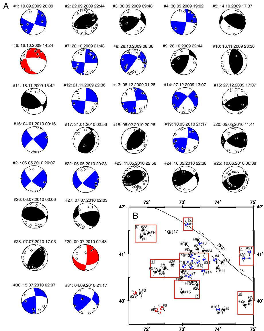
Figure 4 Fault plane solution catalog with picked polarities. (A) Fault plane solutions derived in this study (based on first motion polarities), color coded by their mechanism (black = thrust mechanism, blue = strike-slip mechanism, red = normal mechanism) with picked polarities plotted on the focal mechanisms (black dots correspond to positive polarities; white dots correspond to negative polarities), labeled as shown in Table 3. (B) Map view of fault plane solutions derived in this study (based on first motion polarities and moment tensor inversion), labeled as shown in Tables 3 and 4.
