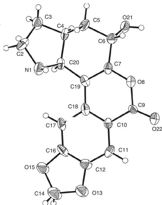
Fig. 1. ORTEP derived from the single-crystal X-ray analysis of compound 20 (CCDC no. 944982) with labelling of selected atoms. Anisotropic displacement ellipsoids display 30 % probability levels. Hydrogen atoms are drawn as circles with small radii.
