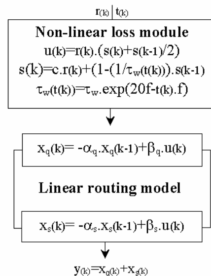
Figure 1. The IHACRES model.
