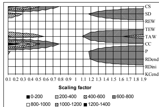
Figure 4. Contour plot of deep drainage (in mm) with changes in CATCHCROP model parameter values.
