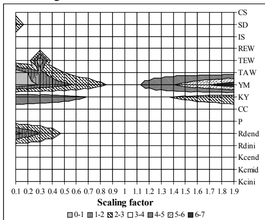
Figure 3. Response in crop yields to changes in CATCHCROP model parameters for paddy rice on land unit 88.
