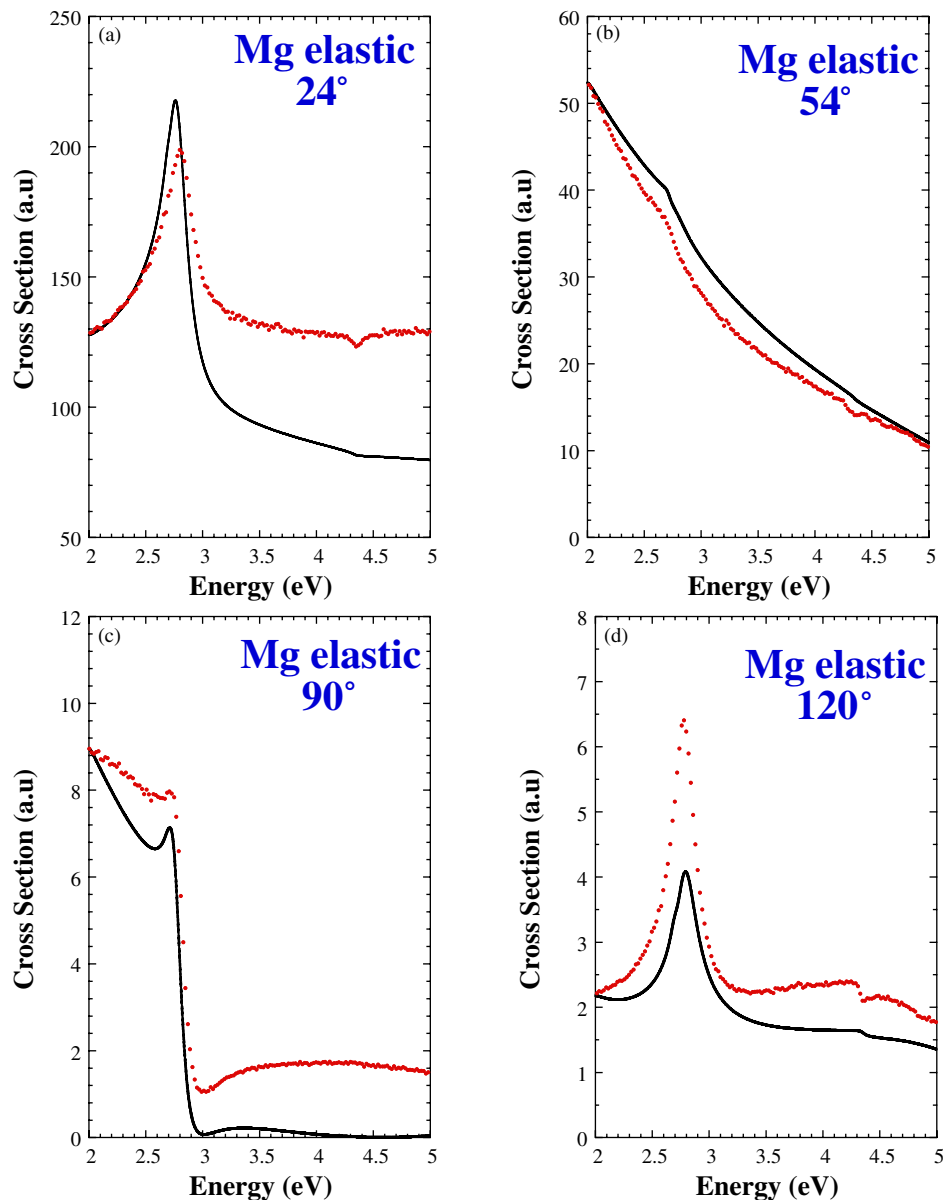
Figure 4. Comparison of experiment and theory (solid line) for elastic electron scattering from Mg at (a) 24°, (b) 54°, (c) 90° and (d) 120°. In each case, the experiment has been normalized to the theory at an energy of 2 eV. The vertical scale is in atomic units (a.u.).
