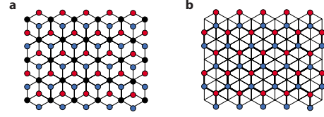
FIG. 5. (Color online) (a) Tight-binding model of a flake of bilayer graphene, consisting of a top and a bottom layer where each layer accommodates a honeycomb lattice of carbon atoms. Black dots denote dimer sites, where carbon atoms of both layers lie on top of each other and are coupled with interlayer coupling constant \gamma_1 . Light (red and blue) dots denote sites of isolated carbon atoms (either on the top or the bottom layer). Lines denote intralayer nearest-neighbor hopping with coupling constant \gamma_0 . (b) Effective model for the two low-energy bands, obtained after decimation (algebraic elimination) of the dimer sites. Thick lines denote coupling with strength 2\gamma' while thin lines denote coupling with strength \gamma' , where \gamma' = \gamma_0^2/\gamma_1 .
