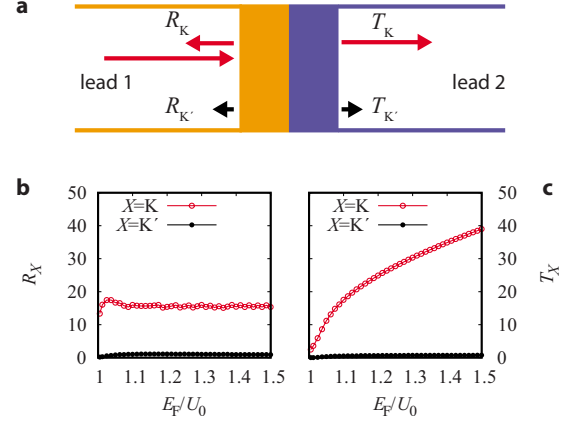
FIG. 2. (Color online) Absence of intervalley scattering. Panel (a): top-view sketch of a (zigzag) graphene nanoribbon geometry with a pseudospin interface, and definitions of reflection and transmission coefficients (summed over all channels) when a K -polarized current is injected into lead 1. Panels (b) and (c): numerical results for the valley-resolved reflection and transmission coefficients (nanoribbon width W \approx 150\hbar / \sqrt{2m|U_0|} ).
