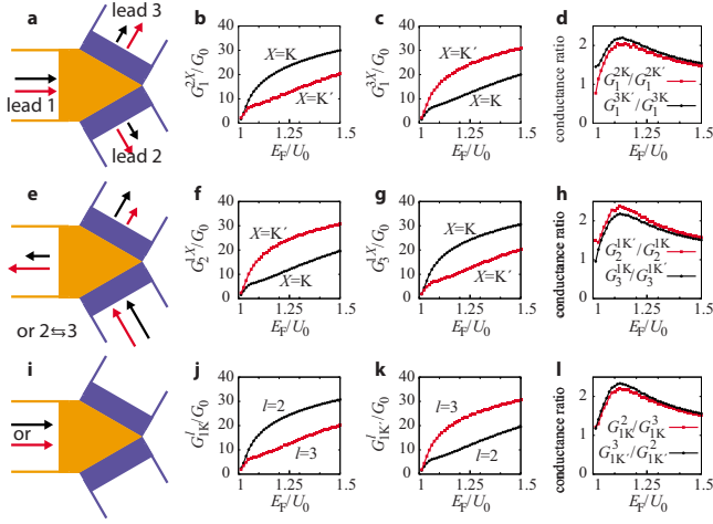
FIG. 3. (Color online) Valleytronics applications. Panel (a): top-view sketch of a valley splitter, consisting of a Y junction where electrons are injected through lead 1, and collected in leads 2 and 3. In this setup, the contact region has the same gate polarity as lead 1, and the incoming current in this lead is valley unpolarized. Panels (b) and (c): valley-resolved conductance of electrons in leads 2 and 3. Panel (d): ratio of the larger to the smaller conductance in these two leads. Analogously, panels (e)–(h) demonstrate that valley polarization can be created in lead 1 by injecting unpolarized currents into lead 2 or 3. Panels (i)–(l) show how the total current in leads 2 and 3 can be used to detect the valley polarization of an incoming current in lead 1.
