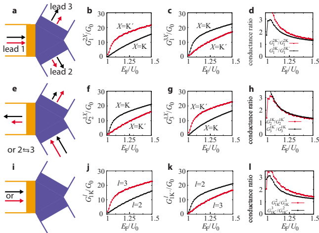
FIG. 4. (Color online) Alternative design of the valley splitters, polarizers, and detectors of Fig. 3, where the contact region has the same gate polarity as leads 2 and 3. Qualitatively, the results for valleys K and K' are now interchanged; however, the influence of edge states between leads 2 and 3 result in a notable lead asymmetry of the conductance ratios.
