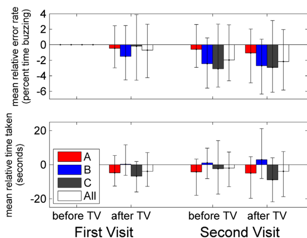
Figure 6. Visuomotor coordination.
