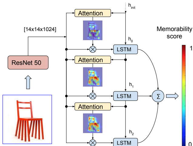
Figure 1: AMNet iteratively generates attention maps linked to the image regions correlated with the memorability. After three iterations the memorability scores are added and presented on the output.
