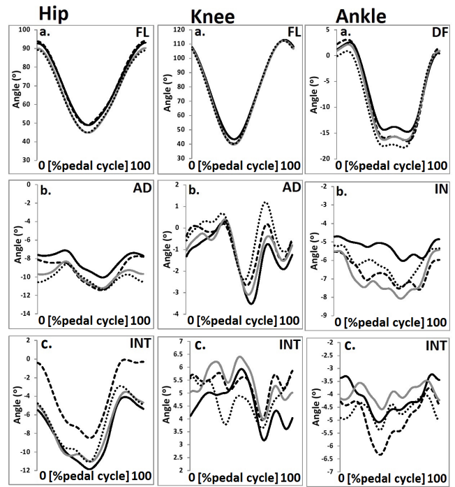
Figure 1. Hip, knee and ankle joint kinematics at 110 RPM as a function of orthotic condition in the a. – sagittal, b. – coronal and c. – transverse planes
