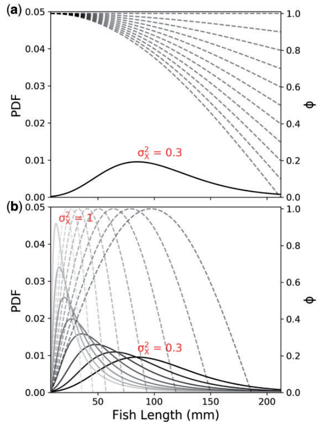
Figure 4. Length class weighting ( \phi ; proportion of gas-bladdered fish by length class, shown by dashed line) for scenarios 2 (a) and 3 (b). (a) Single log-normal distribution plotted ( \mu = 0 , \sigma_X^2 = 0.3 ), \phi is plotted over a range of \phi_{\min} values between 0 and 1. (b) Log-normal distributions scaled to fish length class, where the mean was set to 0 and the variance ( \sigma_X^2 ) ranged from 0.3 to 1. \phi plotted for each distribution. Maximum value of x-axis set to L = 212 mm, which is the length class at the 97.5th percentile of the broadest log-normal distribution ( \mu = 0 , \sigma_X^2 = 0.3 ).
