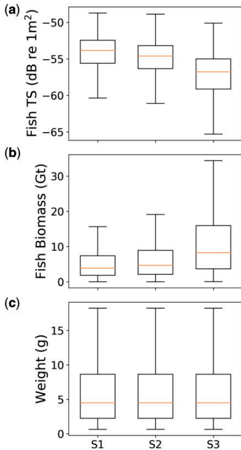
Figure 5. Summarized mesopelagic fish biomass model results for each scenario. (a) Mean fish TS = 10 \log_{10}(\overline{\sigma_{bsf}^2}) , (b) global fish biomass, and (c) mean individual fish weight. Scenario 1 (S1) all fish have gas bladders, whereas in scenarios 2 (S2) and 3 (S3), a proportion of fish are without gas bladders. Horizontal line within each box is the median value, box limits are the inter-quartile range, i.e. 25 and 75% quantiles. The whiskers (vertical lines) are 1.5 times the inter-quartile range. Outliers not plotted.
