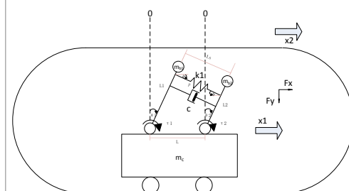
Fig 2: The Proposed Capsule Robot System 2
