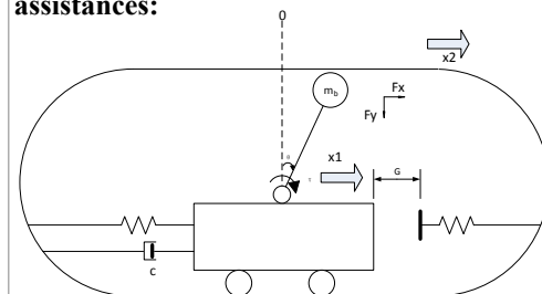
Fig 1: The Proposed Capsule Robot System 1
