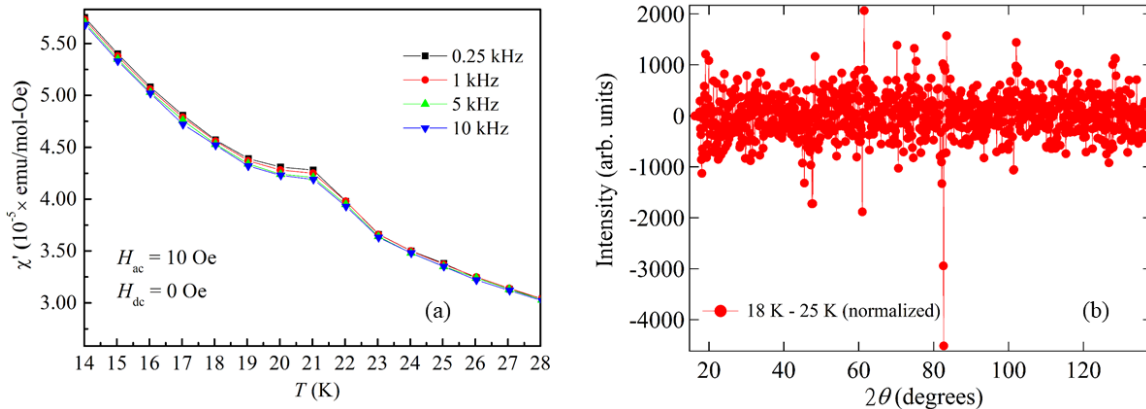
FIG. 6. (a): Temperature variation of ac susceptibility of \text{Nd}_2\text{Ru}_2\text{O}_7 at various frequencies with an ac field of 10 Oe. The position of the peak at 21 K does not change with the frequency of the ac field. H_{dc} = 0\text{ Oe} . (b) The difference data of I(18\text{ K}) - I_{\text{normalized}}(25\text{ K}) . No magnetic peaks are observed in the difference data indicating there is no discernable change in the magnetic structure around 21 K.
