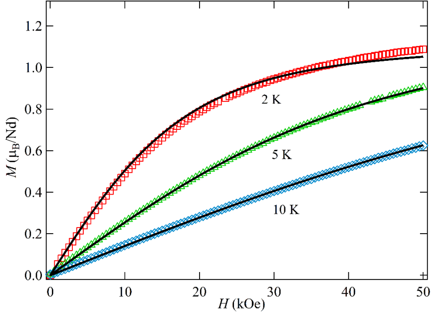
FIG. 3. Isothermal magnetization versus field curves of \text{Nd}_2\text{Ru}_2\text{O}_7 for a magnetic field H \leq 50 kOe measured at T = 2 , 5, and 10 K. The solid curves represent fits of the M(H) data using equation (1).
