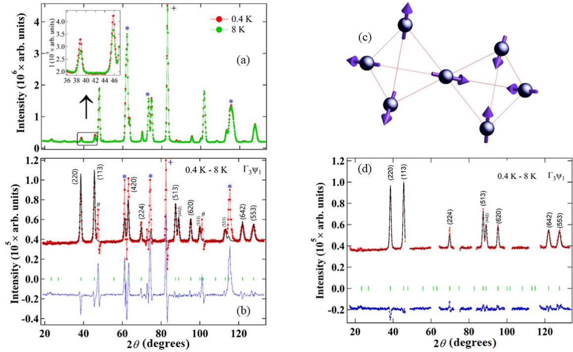
FIG. 5. (a) Neutron diffraction pattern of Nd 2 Ru 2 O 7 recorded at 0.4 and 8 K. (b) Rietveld refinement of the magnetic structure of Nd 2 Ru 2 O 7 at 0.4 K (after subtracting the 8 K nuclear pattern), where the observed data is shown in red, the black line is the theoretically calculated intensity, and the blue line shows the difference between the two. The green vertical lines indicate the positions of the Bragg peaks in the diffraction pattern. The neutron data are best modelled by the irreducible representation \Gamma_3 with an all-in-all-out spin configuration of the Nd 3+ ions. The peaks at 61°, 74°, and 115° (denoted by *) are due to scattering from Al in the sample environment, the peak at 83° (denoted by +) is due to the Cu sample holder. The peaks have been shifted upwards by 20000 for clarity. (c) The all-in all-out configuration of the magnetic moments. (d) Magnetic structure refinement profile of Nd 2 Ru 2 O 7 at 0.4 K (after subtracting the 8 K nuclear pattern), where the regions with background peaks have been excluded. The neutron wavelength used was 2.41 Å.
