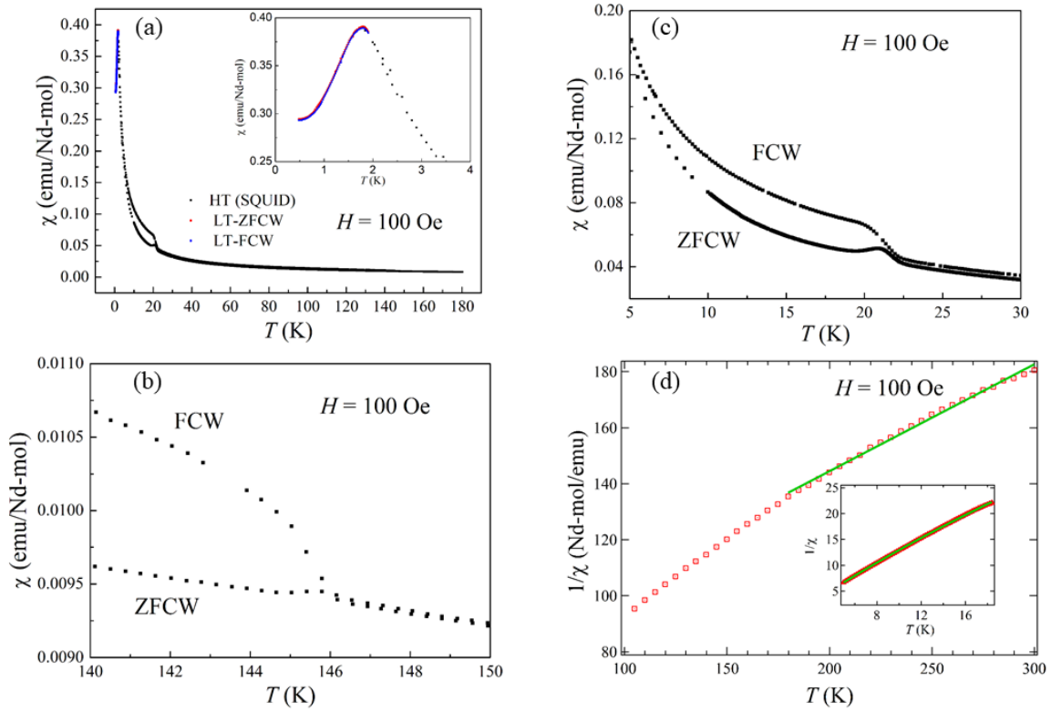
FIG. 2. (a) Temperature variation of the dc magnetic susceptibility of \text{Nd}_2\text{Ru}_2\text{O}_7 at H = 100 Oe in the temperature range 0.4 to 190 K. Three features are observed at 1.8, 21, and 146 K. The inset shows the peak at 1.8 K in more detail. The high temperature (HT) data is taken with an MPMS SQUID magnetometer and the low temperature (LT) data is taken in the same system with a ^3\text{He} insert. ZFCW and FCW indicate the zero-field-cooled warming and field-cooled warming data respectively. (b) Ordering of the \text{Ru}^{4+} 4d moments leads to a cusp-like anomaly in the ZFCW magnetic susceptibility and a splitting of ZFCW and FCW curves around 146 K. (c) Temperature variation of the dc magnetic susceptibility of \text{Nd}_2\text{Ru}_2\text{O}_7 showing the anomaly at 21 K due to weak ferromagnetic ordering of the \text{Nd}^{3+} and \text{Ru}^{4+} ions. (d) Temperature variation of inverse susceptibility in the temperature range 100 \leq T \leq 300 K. The solid line shows a fit to the Curie-Weiss law. The inset shows the inverse susceptibility in the temperature range 5 \leq T \leq 18 K, where the solid line shows the fit to a modified Curie-Weiss law i.e., \chi(T) = \chi_0 + C/(T - \theta_{cw}) .
