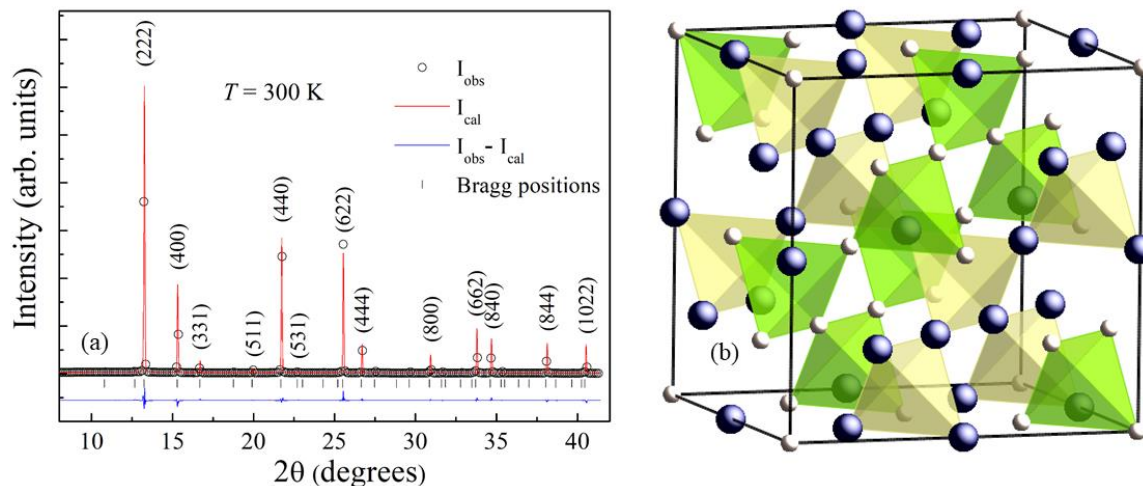
FIG. 1. (a) Rietveld refinement results of the powder x-ray diffraction pattern of \text{Nd}_2\text{Ru}_2\text{O}_7 at room temperature. The open circles show the observed intensity data, the red line indicates the theoretically calculated intensity, and the blue line represents the difference between the observed intensity and calculated intensity. The vertical bars mark the Bragg-peak positions. The wavelength of x-rays used is 1.54 \text{ \AA} . (b) An illustration of the double pyrochlore structure formed by two types of tetrahedra where one type of tetrahedron has Nd atoms at its corners (shown by the large grey spheres) and the other tetrahedra have Ru atoms at the corners (shown by the small white spheres).
