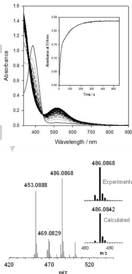
Figure 1. a) UV-Vis absorption spectral monitoring of the formation of 3 upon reaction of 1 (0.3 mM) with 10 equiv H 2 O 2 in acetonitrile at -40 °C. Inset: kinetic trace at 514 nm. b) CSI-MS of 3 generated by adding H 2 O 2 (10 equiv) to 1 in acetonitrile at -40 °C. The peak at m/z 453.0888 corresponds to the starting iron(II) complex [[Fe II (PyNMe 3 )](CF 3 SO 3 ) + . Inset: calculated spectra for [[Fe III (OOH)(PyNMe 3 )](CF 3 SO 3 ) + with m/z = 486.0842 and comparison with the experimental pattern.
