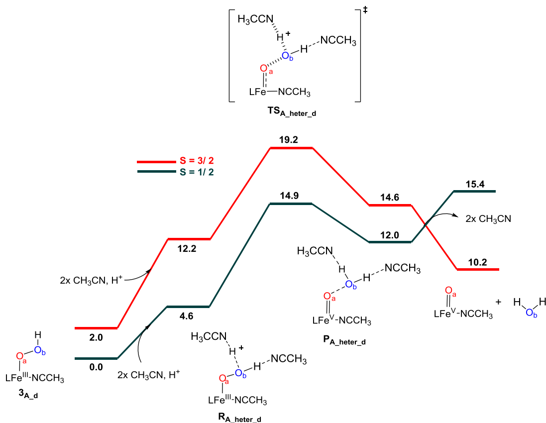
Figure 6. Free energy profile of the acid-triggered acetonitrile-assisted heterolytic O–O bond cleavage mechanism at -40\text{ }^{\circ}\text{C} in compound 3 ( S = 1/2 and S = 3/2 spin surfaces are shown). The \text{PyNMe}_3 ligand is represented by label 'L'
