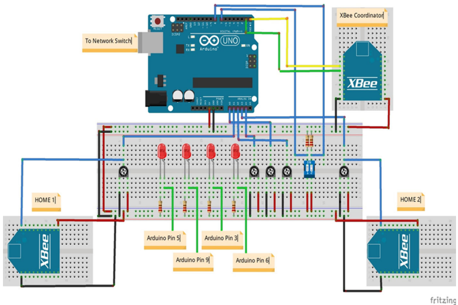
Fig. 3 Circuit diagram
