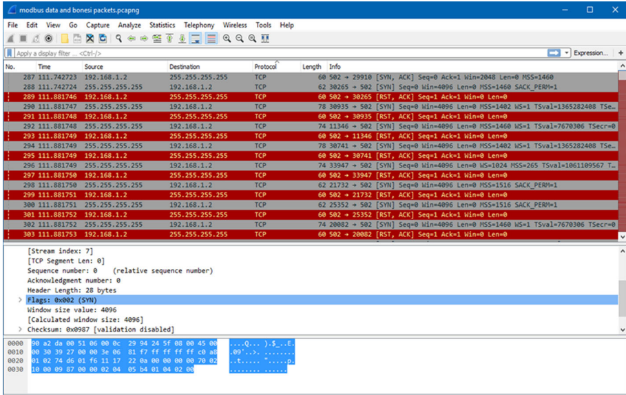
Fig. 16 Wireshark showing captured DoS SYN packets
