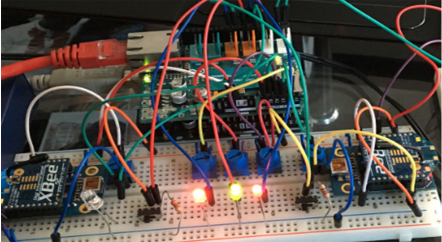
Fig. 6 Arduino board as a PLC
