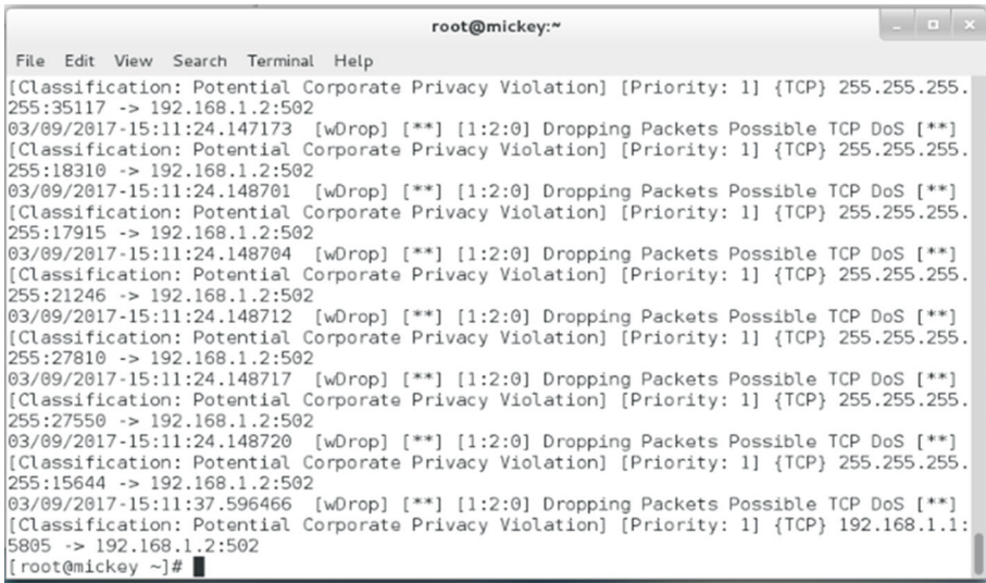
Fig. 19 Suricata NIPS dropping attack packets
