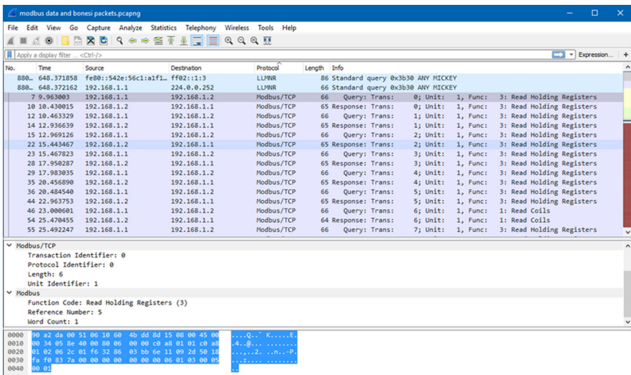
Fig. 11 Wireshark showing exchange of Modbus TCP request and response packets
