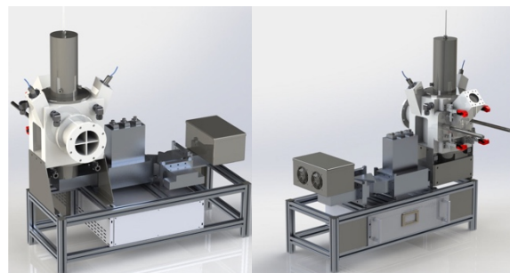
Figure 2: Industrial bespoke microwave heating apparatus
