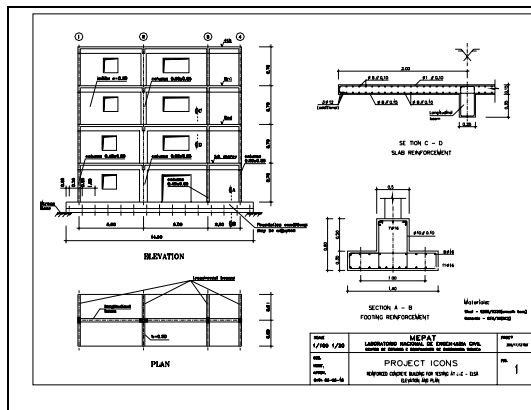
Fig. 1: Plan and elevation views of concrete frame plus masonry infill building
