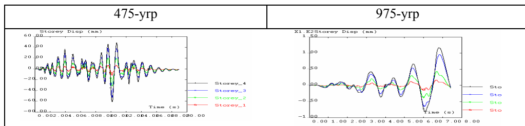
Fig. 6: Storey Displacements
