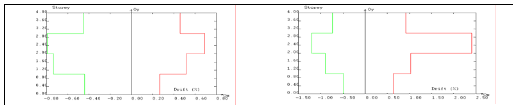
Fig. 7: Maximum Drift Profiles
