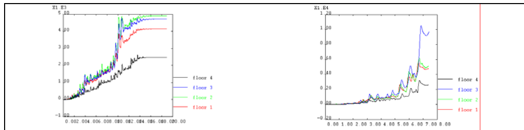
Fig. 8: Dissipated Energy (kNm)
