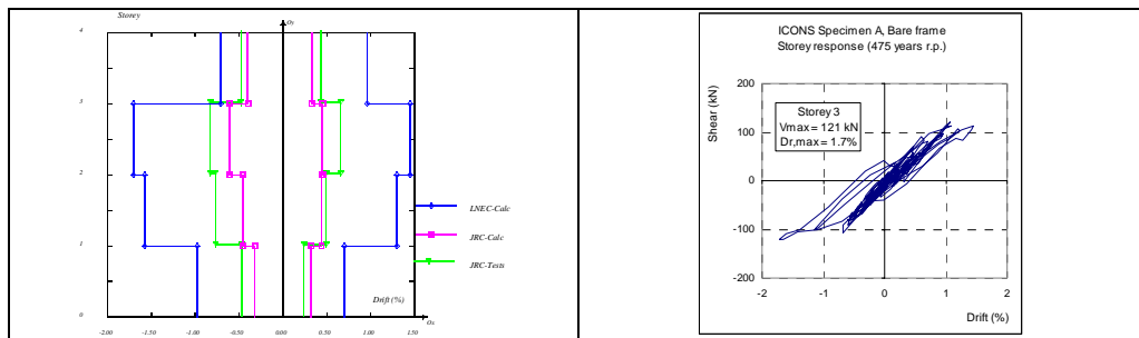
Fig. 10: Drift profiles (numerical and experimental)
