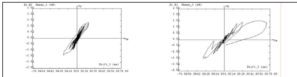
Fig. 9: 3 rd Storey Shear/Drift diagram
