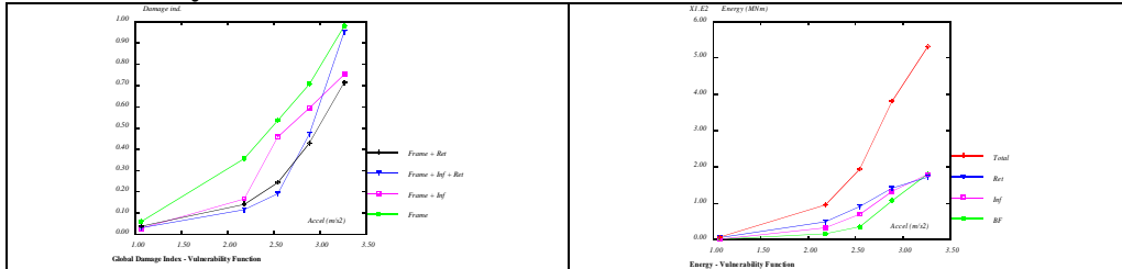
Fig. 4: Global damage on the frame structure (evolution with input intensity)
