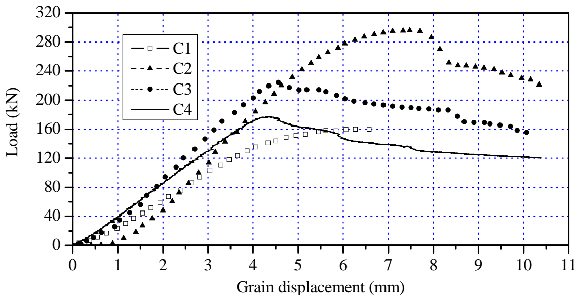
Fig. 3 – Grain displacement - load curves obtained in the compression tests
