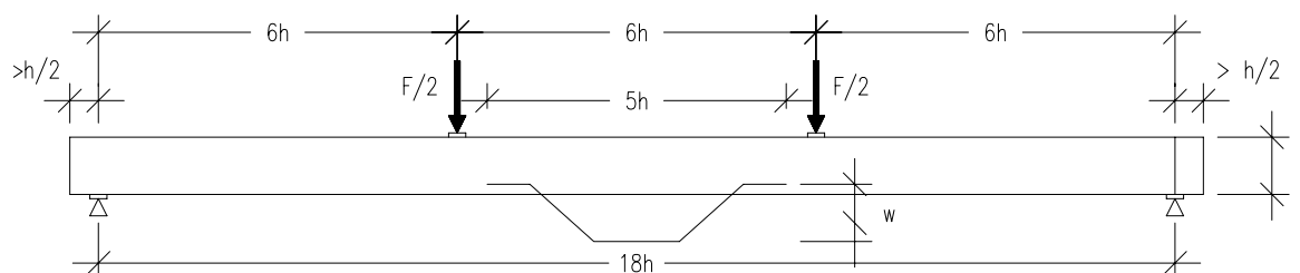
Fig. 1 - Test arrangement of the bending test
