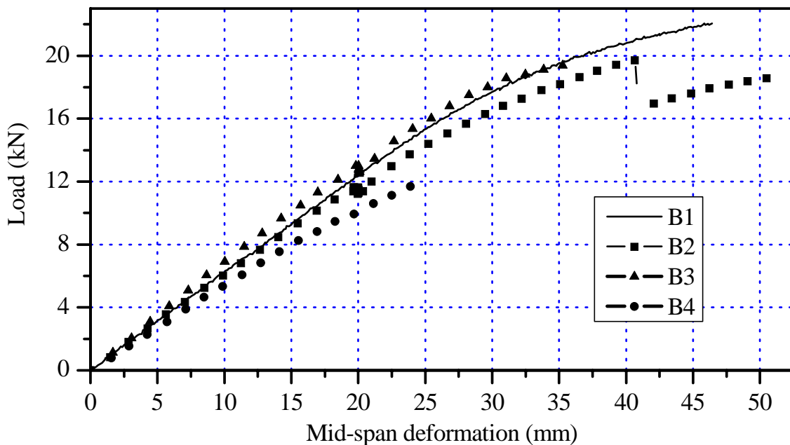
Fig. 2 – Mid-span deformation vs load curves obtained in the bending tests
