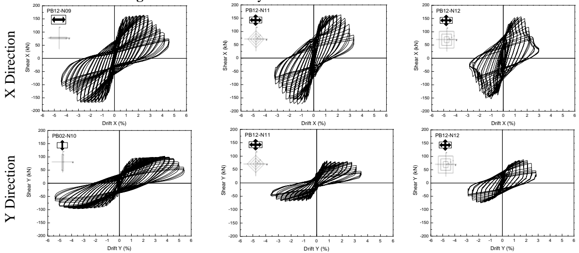
Figure 5. Shear-Drift hysteretic curves for columns N09 to N12
