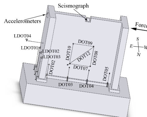
Fig. 1. Adobe wall schematics with indication of the sensors location.
