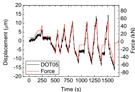
Fig. 2. Displacement evolution measured at sensor DOT05 placed at the base of the N face of the wall and applied force history.
