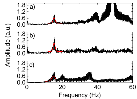
Fig. 3. Frequency spectrum obtained by Fourier transform of the acceleration data over time in the dynamic test 5: (a) Optical Accelerometer, (b) Electronic Accelerometer and (c) Seismograph.
