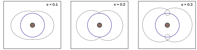
Fig. 4. Typical path of a Plutino (dotted line) in the rotating frame of Neptune (full line) for different eccentricity values ( e = 0.1, 0.2 and 0.3 ). Only high eccentricity values ( e > 0.2 ) allow the Plutino to cross the orbit of Neptune. Due to the 3:2 mean motion resonance the trajectories are repeated every two orbits of the TNO around the Sun.
