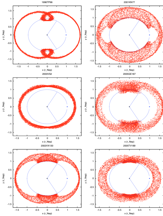
Fig. 6. Orbital evolution of some Plutinos (in red) taken from Table A.4 over 100 Myr in the co-rotating frame of Neptune (in blue). Each panel shows the projection of the TNO position every 10 kyr in the orbital plane of Neptune. x and y are spatial coordinates centered on the star and rotating with Neptune, normalized by the Neptune-Sun distance. We have chosen the most representative cases, namely, Plutino 1996TP66, with the lowest libration amplitude ( \Delta\varphi = 7.2^\circ , e = 0.328 , i = 5.6^\circ ), Plutino 2001KN77, with the largest libration amplitude ( \Delta\varphi = 120.4^\circ , e = 0.242 , i = 2.4^\circ ), Plutino 2003VS2, with the smallest eccentricity ( e = 0.072 , i = 14.8^\circ ), Plutino 2005GE187, with the highest eccentricity ( e = 0.329 , i = 18.2^\circ ), Plutino 2002VX130, with the smallest inclination ( e = 0.220 , i = 1.3^\circ ), and Plutino 2005TV189, with the highest inclination ( e = 0.186 , i = 34.5^\circ ).
