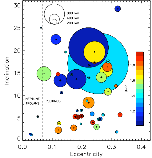
Fig. 1. Orbital inclination vs. eccentricity, estimated size, and color of Neptune Trojans and Plutinos for which those properties have been measured.
