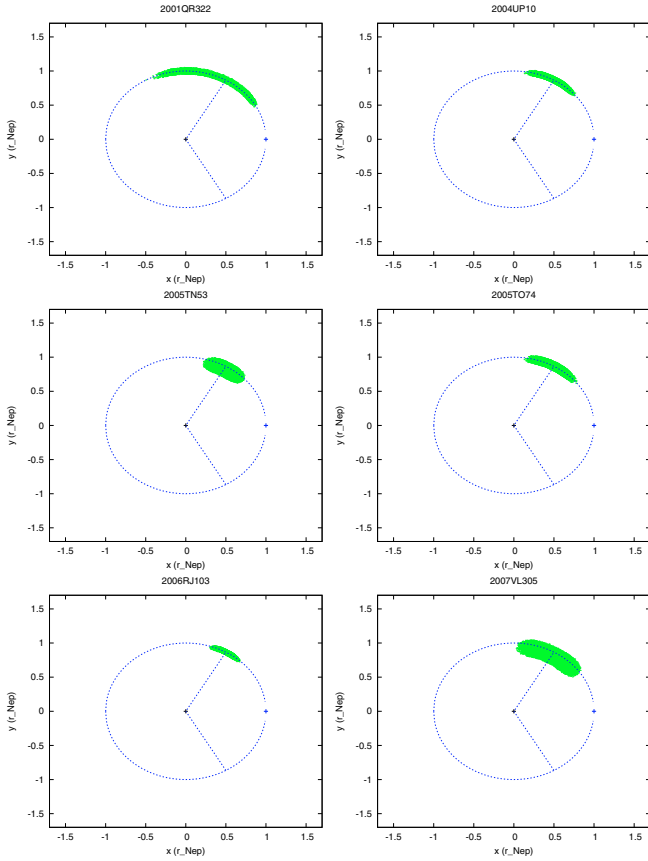
Fig. 3. Orbital evolution of the Neptune Trojans (in green) listed in Table A.3 over 100 Myr in the co-rotating frame of Neptune (in blue). Each panel shows the projection of the TNO position every 10 kyr in the orbital plane of Neptune. x and y are spatial coordinates centered on the star and rotating with Neptune, normalized by the Neptune-Sun distance. All Trojans orbit around the Lagrangian point L_4 and execute tadpole-type orbits. More scattered orbits correspond to higher values of the eccentricity and inclination, while distance to the L_4 point depend on the libration amplitude.
