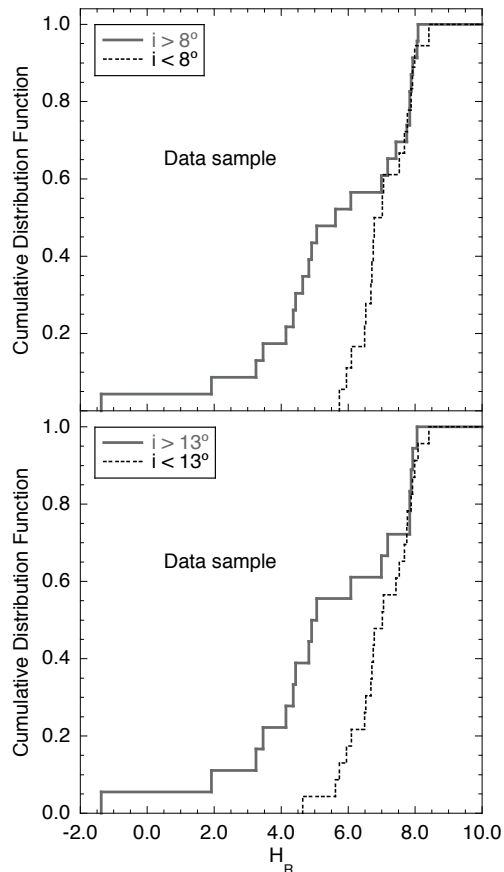
Fig. 2. Cumulative distribution function of absolute magnitudes H_R for Plutinos above and below 8^\circ of inclination ( top ) and Plutinos above and below 13^\circ ( bottom ). The incompatibility of distributions between the higher and lower inclined Plutinos is similar in both cases. There is an evident lack of intrinsically bright (large) objects among the low-inclined Plutinos.
