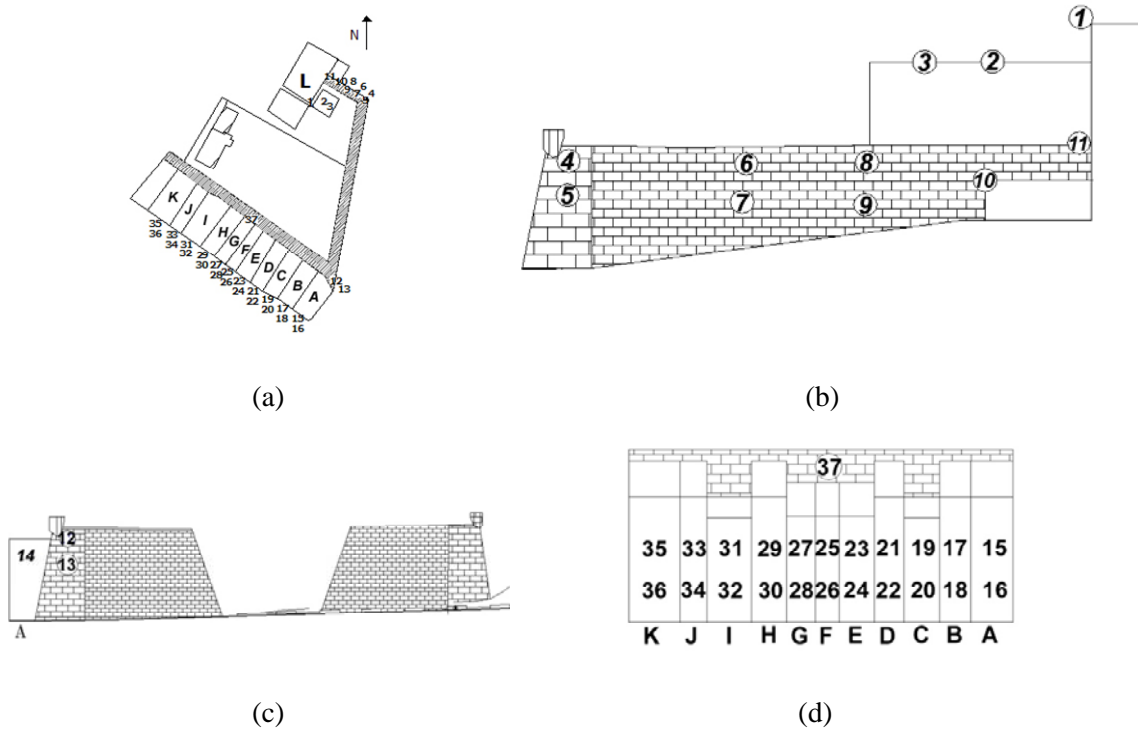
Figure 8. Key-points location and controlled buildings: a) Plan view; b) NE wall, Manas stair; c) SE wall, 25 de Abril road; d) SO wall and attached buildings (from A to K), Sol road
