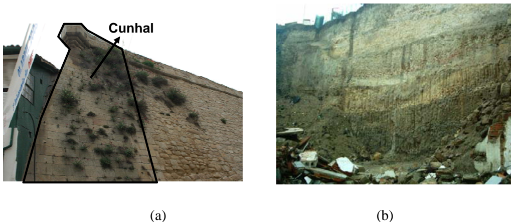
Figure 4. a) Cunhal that connects the SE and SW walls; b) Soil profile supported by the wall (December 2005)
