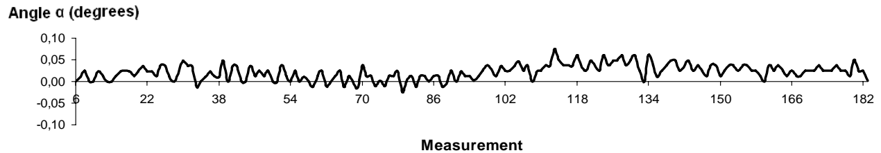
Figure 17. Evolution of \alpha for the alignment defined by the key points 6 and 7 of the NE wall
