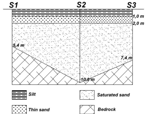
Figure 5. Results of the exploration drilling tests done in the downstream side of the SE wall (Tested by Material and Soils Laboratory of UTAD)
