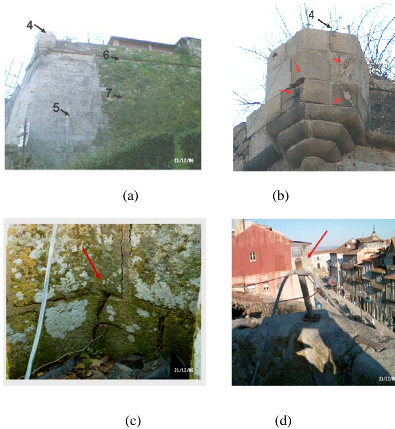
Figure 16. Key point 4: Some pathologies existing around the key point 4 and resulted from the working tasks related to the reconstruction process: a) Location of the key points 4, 5, 6 and 7; b) Existing pathologies surrounding the key point 4; c) Existing pathologies surrounding the key point 4; d) Existing steel bar next to the key point 4
