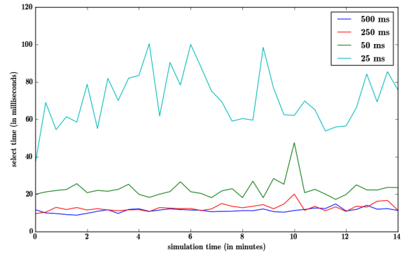
Fig. 5. CouchDB: Item retrieval with simultaneous Item insertions
