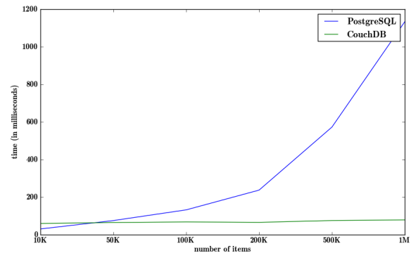
Fig. 2. PostgreSQL vs CouchDB: Item retrieval
