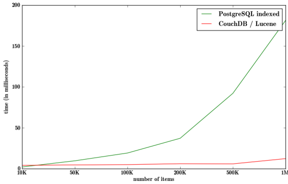
Fig. 3. PostgreSQL vs CouchDB / Lucene: Item searching
