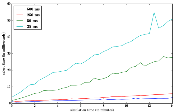
Fig. 4. PostgreSQL: Item retrieval with simultaneous Item insertions
