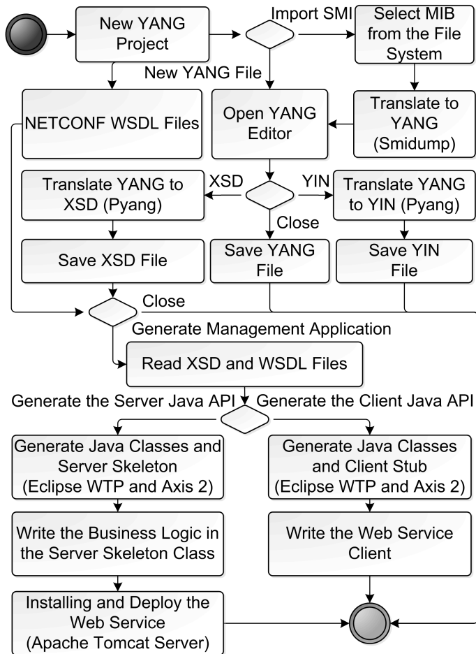
Figure 1: Development Activity Diagram
