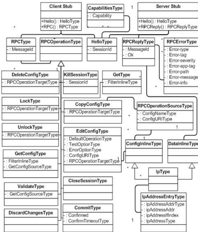
Figure 6: Class diagram of the generated classes
