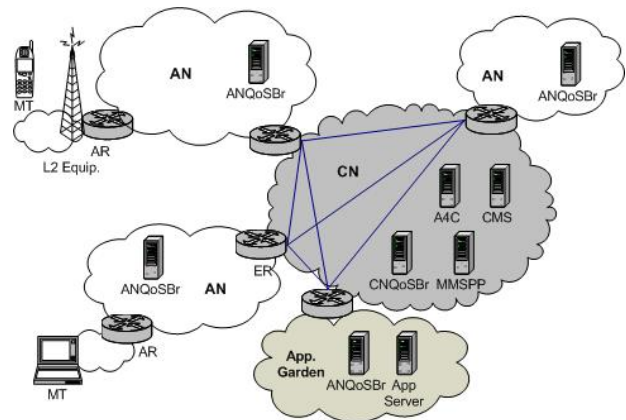
Figure 2 – Daidalos' Architecture.
