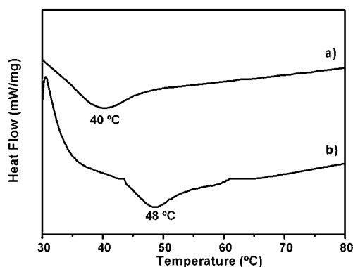
Fig. 8 DSC of (a) Ag/PtBA nanocomposites and (b) PtBA , both prepared by miniemulsion polymerization.
