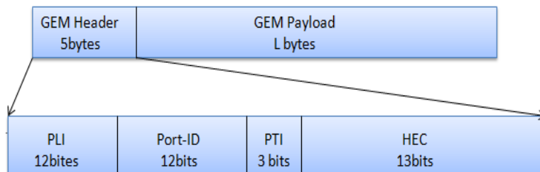
Figure 3.10: G-PON GEM frame [G.984.3, 2008].
