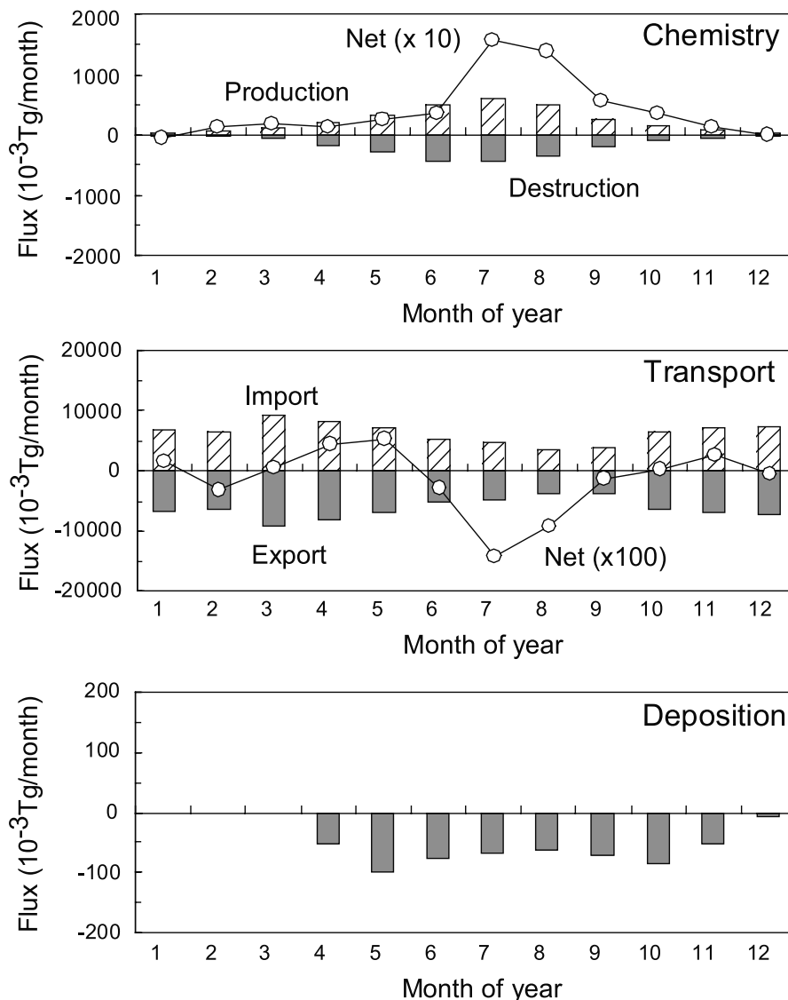
Figure 8. Same as Figure 7, but for O 3 , note that the scale for transport (middle panel) is one order of magnitude larger than that of chemistry (upper panel).
