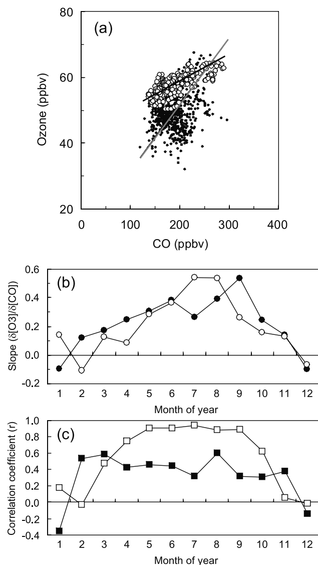
Figure 5. (a) Scatterplots of O 3 to CO observed in April 2000 (solid circles) and predicted by the model in April (open circles). One-hour averages and 3-hour averaged surface mixing ratios are shown from the observations and the model, respectively. RMA regression lines are included for each data set (black for the model, and gray for the observations). (b) Seasonal variation of the monthly O 3 -CO slope derived from the observation (solid circles) and the model (open circles). (c) Seasonal variation of the monthly O 3 -CO correlation coefficient ( r ) from the observations (solid squares) and the model (open squares).
