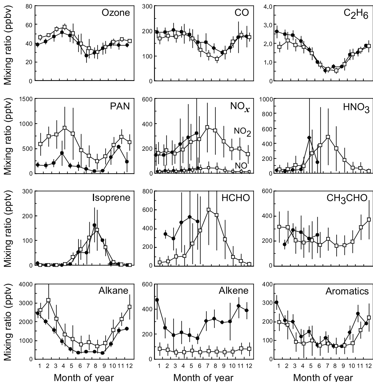
Figure 3. Comparison of observed (solid circles) and modeled (open squares) monthly mean mixing ratios of selected trace gases at Rishiri Island with error bars defining the temporal variability of the time series in each case (as one standard deviation). Modeled mixing ratios are those at the surface level of the Rishiri region. Measured alkanes are the sum of propane, n -butane, i -butane, n -pentane, i -pentane, and n -hexane; alkenes, ethene, propene, and ethyne; aromatics, benzene and toluene.
