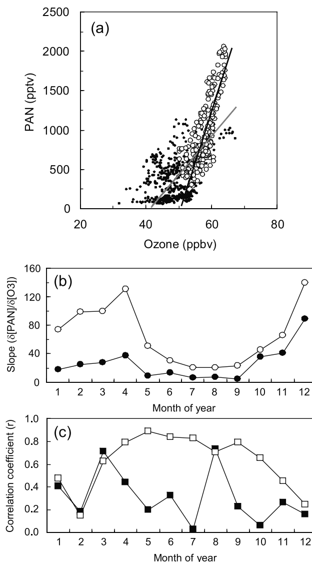
Figure 6. (a) Scatterplots of PAN to O 3 observed in April 2000 (solid circles) and predicted by the model in April (open circles). One-hour averages and 3-hour averaged surface mixing ratios are shown from the observations and the model, respectively. RMA regression lines are included for each data set (black for the model, and gray for the observations). (b) Seasonal variation of the monthly PAN-O 3 slope derived from the observation (solid circles) and model (open circles). (c) Seasonal variation of the monthly PAN-O 3 correlation coefficient ( r ) from the observations (solid squares) and the model (open squares).
