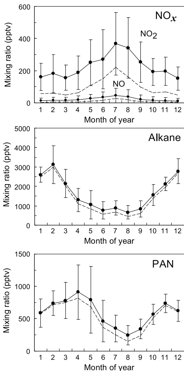
Figure 4. Comparison of the surface mixing ratios of NO x , alkane, and PAN in the model with and without local emissions. Monthly mean mixing ratios (solid circles) with one standard deviation (vertical bars) including emissions are compared to the monthly means without local emissions (dashed line).
