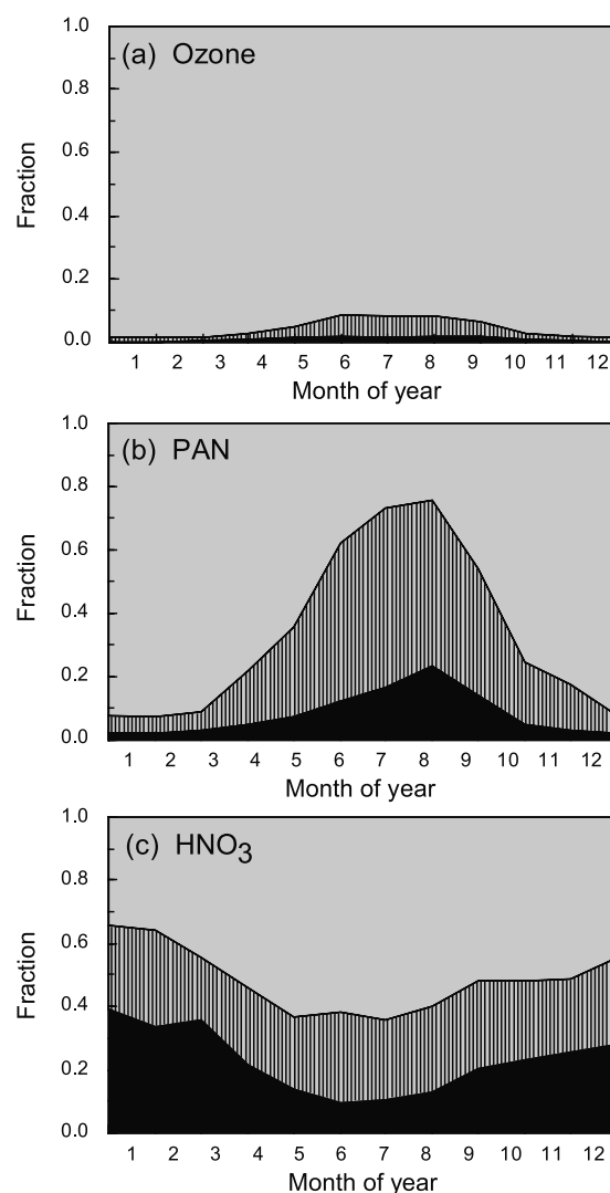
Figure 10. Fraction of transport (gray), and photochemistry from transported precursors (hatched) and local emissions (black) in the seasonal variations of boundary layer (a) O 3 , (b) PAN, and (c) HNO 3 .
