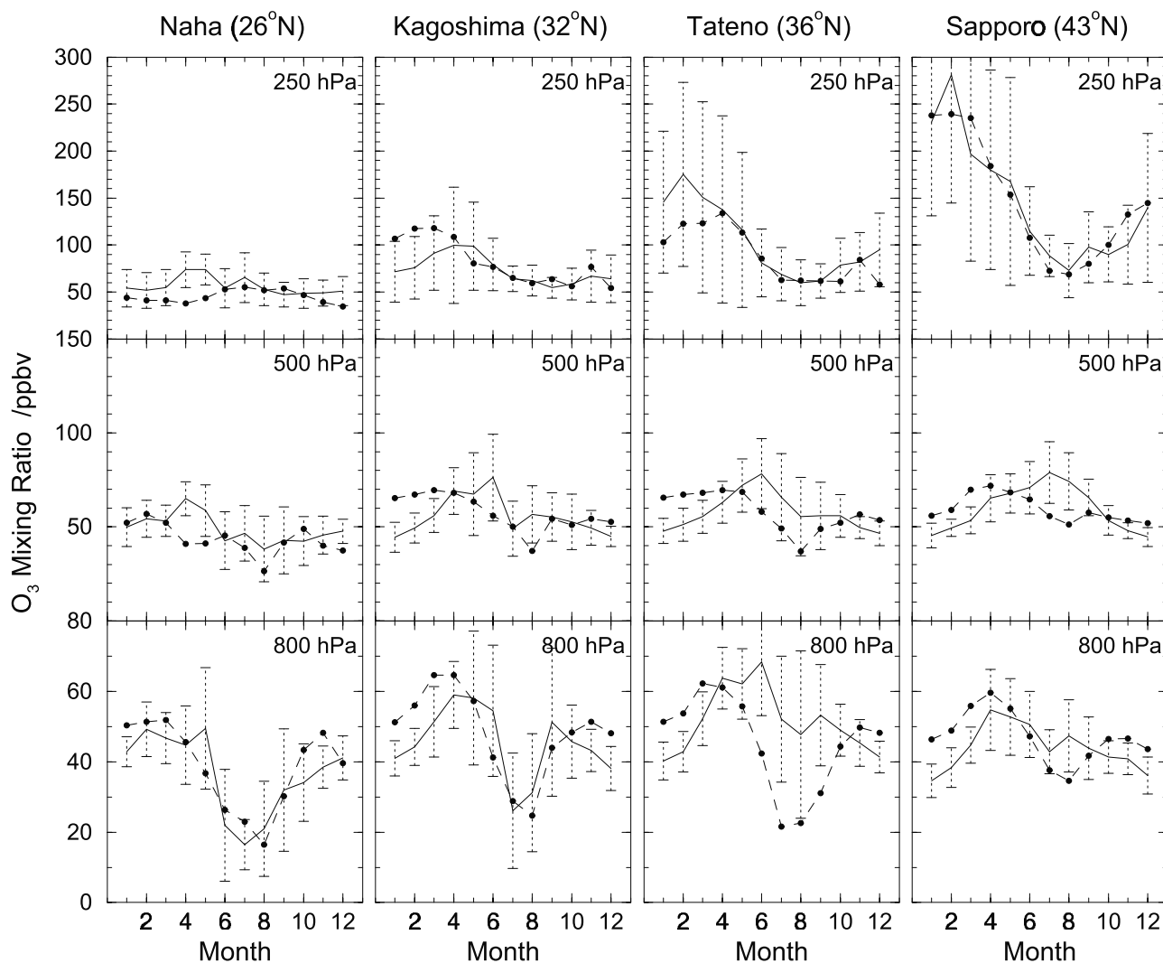
Figure 2. Time series of monthly mean ozone mixing ratios over the period 1980–1995 (1989–1995 for Naha) from ozonesonde measurements over Japan [Logan, 1999] (solid lines), against mean modeled mixing ratios (dashed lines). Error bars define one standard deviation, and reflect the variability during the month over the whole multiyear period.
