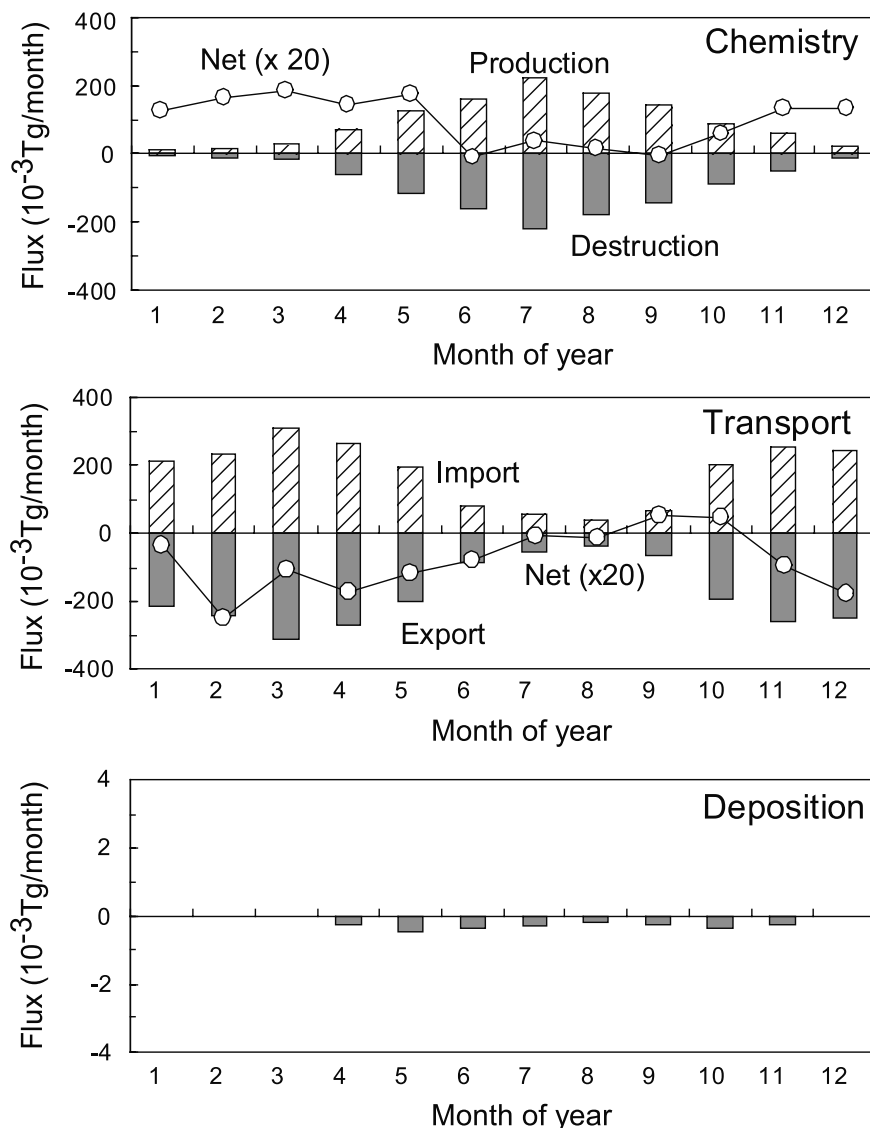
Figure 7. Boundary layer fluxes of PAN for the Rishiri region, separately illustrated for chemistry, transport, and deposition. The contribution from chemistry is separated into chemical production (hatched), chemical destruction (shaded), and net tendency (open circles and lines). The contribution from transport is separated into import (hatched), export (shaded), and net tendency (open circles and lines). Positive values denote import (or chemical production), and negative values export (or chemical loss).
