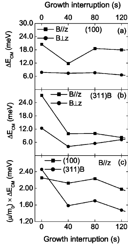
FIG. 4. The PL shift ( \Delta E_{CM} ) as function of the growth interruption for samples with the (100) (a) and (311)B (b) substrate orientations for both B \parallel z (squares) and B \perp z (circles). The product of the effective mass \mu/m_0 and PL shift for B \parallel z , also as a function of growth interruption, is shown in (c) for the (100) (squares) and (311)B (circles) substrate orientations. This product is a measure of the exciton extent. The lines always join the points.
