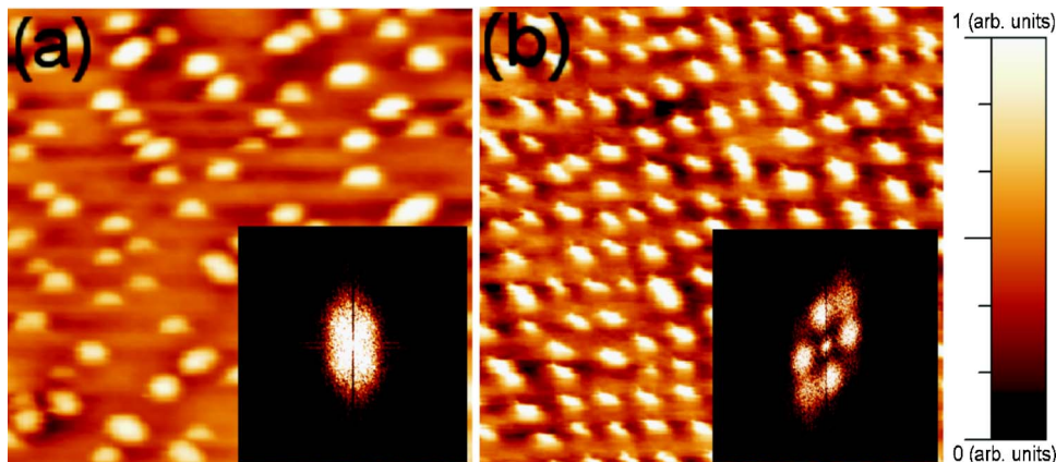
FIG. 4. (Color online) AFM pictures ( 0.5 \times 0.5 \mu\text{m} ) of samples with six stacked layers and (a) a low QD density of 4 \times 10^{10} \text{ cm}^{-2} and (b) a high QD density of 8 \times 10^{10} \text{ cm}^{-2} . Bright areas represent the maximum height of the dots (i.e., about 6 nm). The insets show the corresponding two-dimensional Fourier-transformed pictures, demonstrating the presence of lateral organization only at high QD densities.
