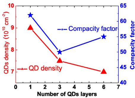
FIG. 3. (Color online) Evolution of the compactness factor and QD density as a function of the number of stacked QDs layers.
