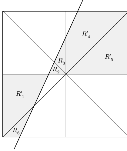
Figure 7: Configuration (3) with median line y = r(x + x(r)) intersecting the square.
