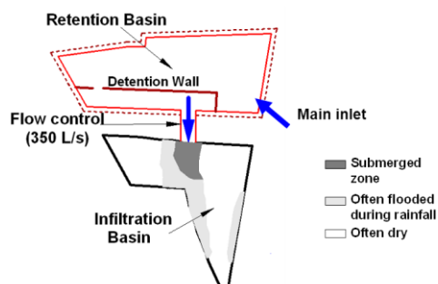
Figure 1. Configuration of the Django Reinhardt retention – infiltration basin and the wet zones distribution in the infiltration basin.
