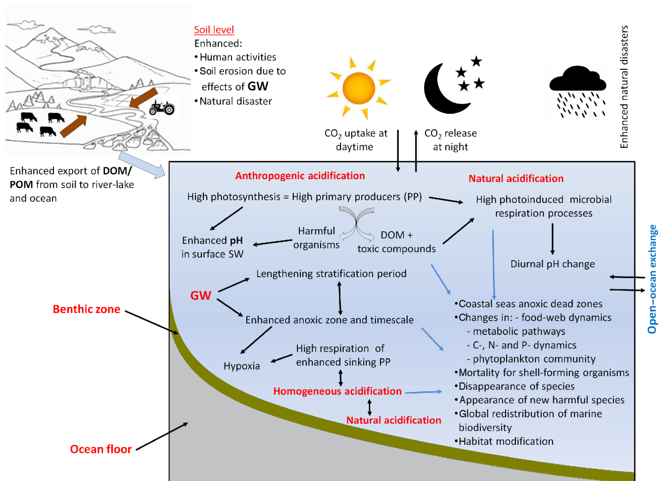
Figure 6. An overview of the potential upcoming ecological and biogeochemical consequences, linking different environmental drivers, processes, and cycles related to acidification in the future ocean.
