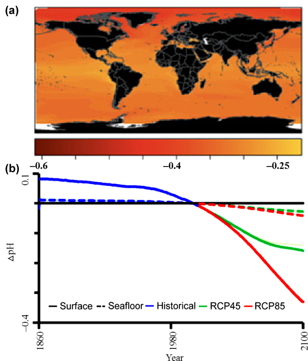
Figure 5. Possible forthcoming changes in pH in the world's oceans. Panel (a) shows the spatial difference between future (i.e., the average from 2091 to 2100) and contemporary (i.e., the average from 1996 to 2005) values under the RCP85 scenario (decadal averages were chosen to minimize aliasing by interannual variability). Aside each color scale the absolute change is provided, whereas the numbers on top indicate the rescaled values; complete results for the RCP85 and RCP45 scenarios for the ocean surface and floor are shown in the reference (Mora et al., 2013). Panel (b) shows the global average change relative to contemporary values under the Representative Concentration Pathways 4.5 (RCP45) and 8.5 (RCP85) scenarios at the ocean surface and seafloor; semi-transparent lines are the projections for the model.
