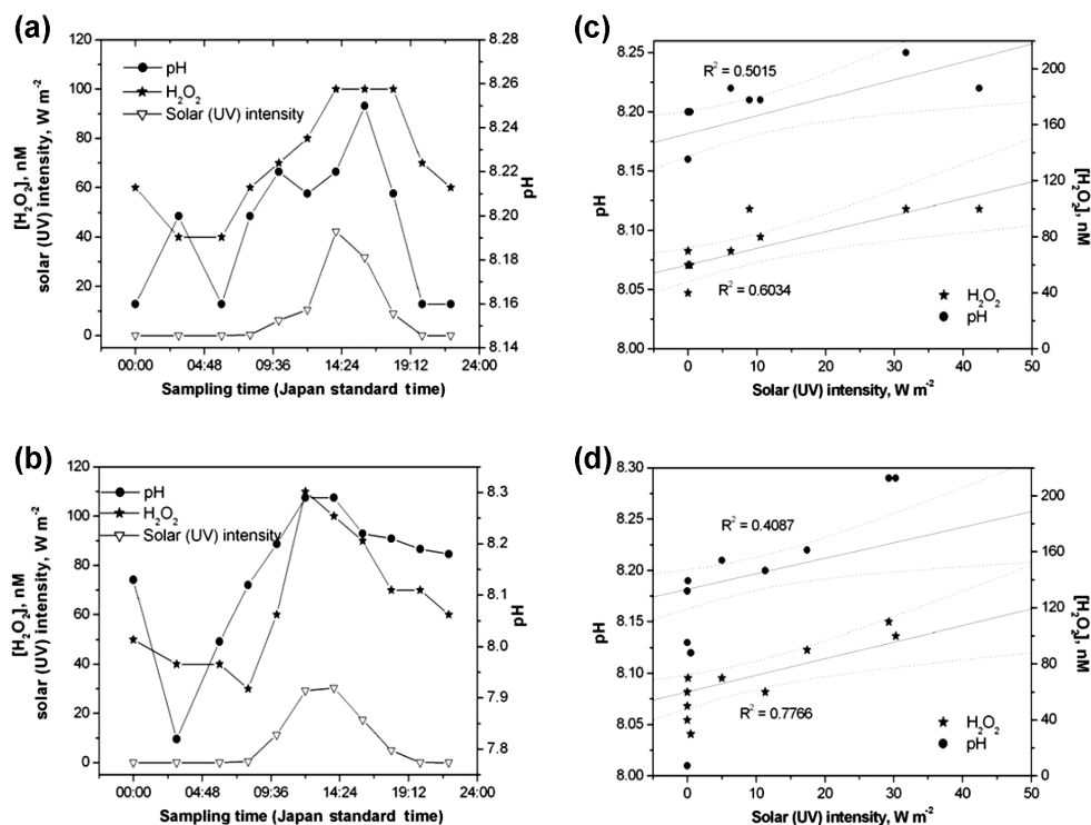
Figure 3. Diurnal changes of pH, \text{H}_2\text{O}_2 and solar (UV) intensity in the seawater of Taira Bay on 9–10 January 2003 (a) and Sesoko Bay on 19–20 January 2003 (b). (c, d): pH and concentration of \text{H}_2\text{O}_2 as a function of the solar UV intensity with the related linear fit regressions in the case of Taira Bay and Sesoko Bay samples, respectively. In the seawater of Taira Bay the pH, \text{H}_2\text{O}_2 , dissolved organic carbon (DOC), and sea surface water temperature (SST) varied in the following ranges: 8.16–8.25, 40–100 nM, 1.14–1.42 ppm, and 18.8–20.9 °C, respectively. In the seawater of Sesoko Bay the relevant ranges were as follows: 7.82–8.28, 30–110 nM, 0.84–1.41 ppm, and 17.7–20.2 °C, respectively.
