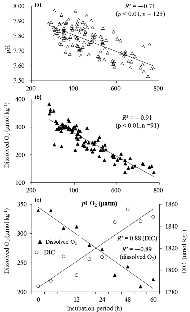
Figure 4. Relationship of p\text{CO}_2[\text{seawater}] with pH (a) and dissolved O 2 (b) in subsurface seawater of the Yellow Sea. Decline in dissolved O 2 combined with an increase in dissolved inorganic carbon (DIC), as a function of the incubation time (60 h), in an experiment conducted using subsurface seawater from the East China Sea (c). Depth ranged from 13 to 75 m for a variety of subsurface seawater samples, with latitudes at 37°25′–39°67′ N and longitudes at 121°16′–124°10′ E. Ten 60 mL bottles for dissolved O 2 and ten 60 mL borosilicate glass bottles for DIC wrapped with black polyethylene were submerged into an in-flow water bath, in which surface seawater was continuously supplied to control the water bath temperature. Dark incubated samples were collected after 12, 24, and 60 h of incubation. Seawater samples for the experiment were collected at 37 m depth on 2 July 2013 using a 10 L Niskin Bottle in the East China Sea at 28°50′ N, 122°15′ E.
