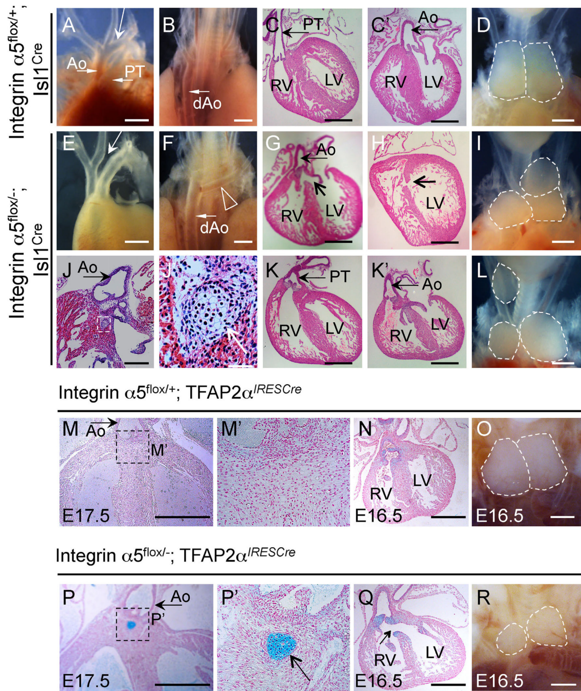
Fig. 9. Cardiovascular and thymus defects in integrin \alpha 5^{flox/-} ; Is11 Cre and in integrin \alpha 5^{flox/-} ; TFAP2 \alpha^{IRESCre} mutants at E16.5 and E17.5. (A–D) Controls; E–L Mutants. (A, E, D, I, L) - ventral views; (B, F) - dorsal views. Ao - ascending aorta; PT - pulmonary trunk; Long arrow in A points to the aortic arch; dAo - descending aorta is marked in (B). (C) PT originates from the right ventricle (RV) in controls; Ao originates from the left ventricle (LV) in controls; (D) two symmetrical thymus lobes of a control embryo are outlined. (E) Arrow points to the missing aortic arch; (F) Arrowhead points to the subclavian artery
