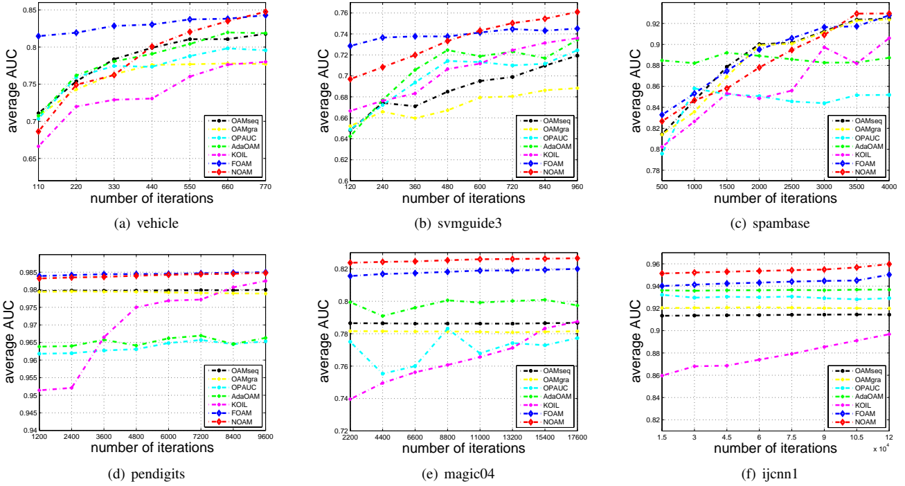
Fig. 1: Evaluation of convergence rate on selected benchmark datasets.
