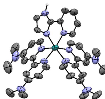
Figure 2. Crystal structure of [\text{Ru}^{\text{NMe}_2}\text{pymH}]^{2+} . Thermal ellipsoids are drawn at the 50 % probability level. Solvent molecules, counter ions and hydrogen atoms, except N-H, are omitted for clarity.
