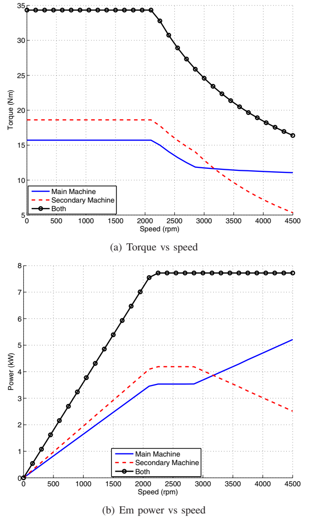
Fig. 6. Torque and power with CPR-MTPA strategy
