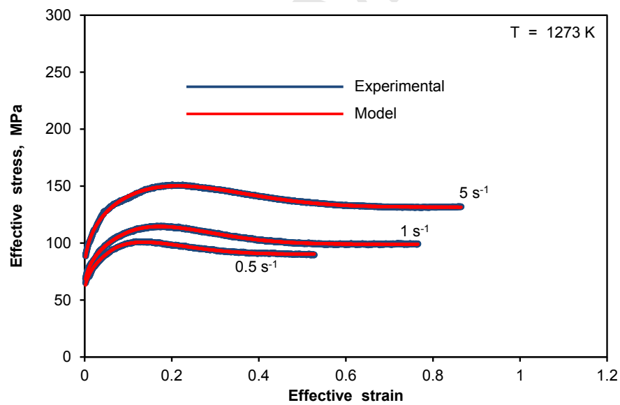
Figure 12: Comparison of the experimental stress-strain curves and the constitutive formulation at 1273 K.
