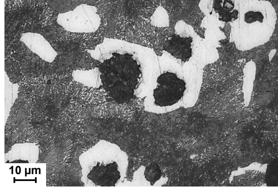
Figure 3: Optical micrograph of the ASTM A536 100-70-03 iron in its original state (etched with saturated nitric acid).
