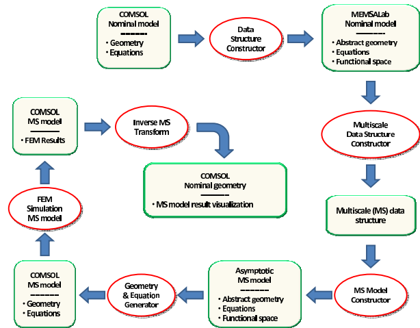
FIGURE 3 – Flowshart of the modelling steps
