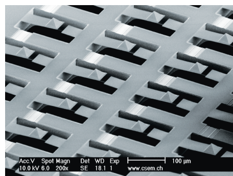
FIGURE 1 – An array of micro-levers for parallel AFM applications. A courtesy of A. Meister from CSEM Switzerland.
