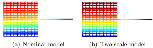
FIGURE 4 – Results for u^0 by FEM simulations
