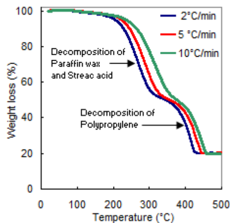
FIG. 2 – Weight binder loss vs. temperature with powder volume loading equals to 60%.
