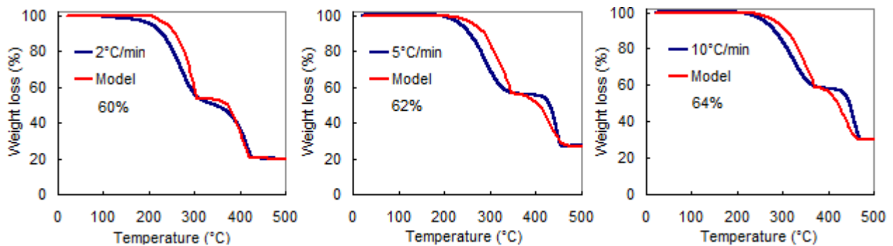
FIG. 6 – Comparison of weight binder loss vs. temperature using both the experiments and the proposed model, for different heating rates.
