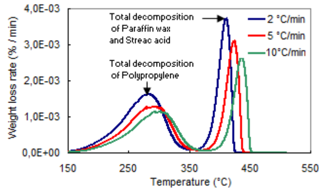
FIG. 3 – Weight binder loss rate at different heating rates with powder volume loading 60%.
