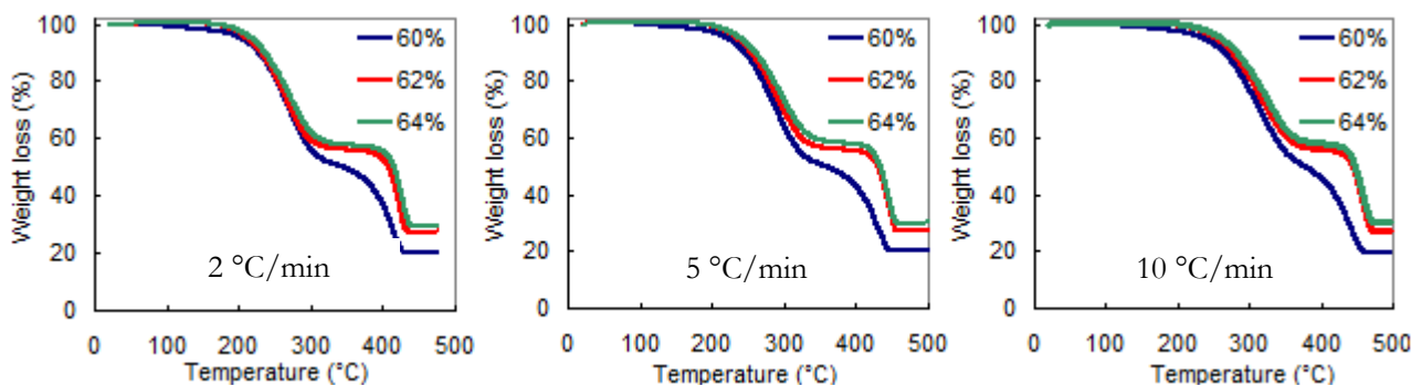
FIG. 5 – Binder loss (in weight) vs. debinding temperature for different powder volume loadings at different heating rates.
