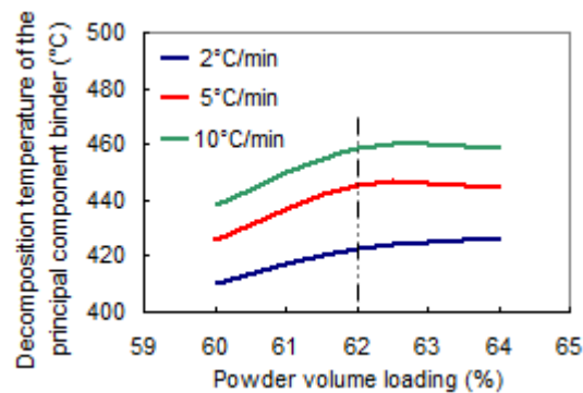
FIG. 4 – Binder decomposition temperature vs. powder volume loading.
