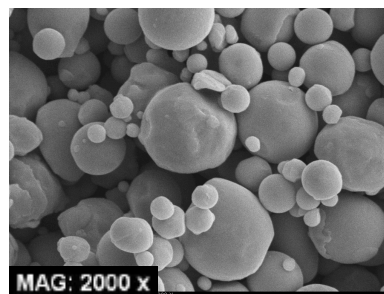
FIG. 1 – SEM photograph of 316L stainless steel powders ( D_{50}=3.4 \mu\text{m} ) used in the proposed investigations.
