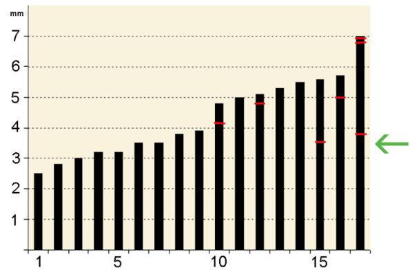
Figure 4: Graphic showing size distribution (max. diameter) of studied Anticalyptrea calyptrata specimens (n=17) from Kaugatuma cliff (lower Pridoli) of Saaremaa and location of the shell repairs (red lines). Green arrow points to the minimum diameter of the shells with repair marks.
