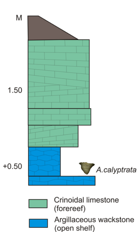
Figure 3: Kaugatuma cliff after EINASTO (1990). Anticalyptrea calyptrata with shell repair occurs in the lower part of section.
