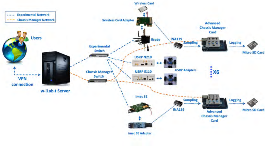
Figure 4.2: w-iLab.t architecture
