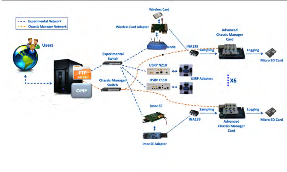
Figure 4.1: NITOS architecture
