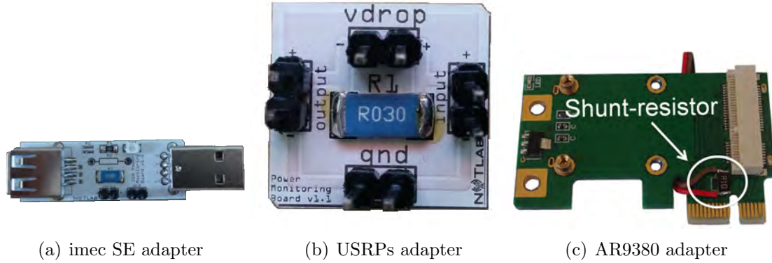
Figure 2.6: Power adapters
