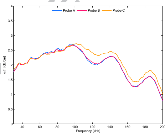
Figure 7: Material attenuation for the non-contact method ( \alpha_{mat}^{(NC)}(f) )
