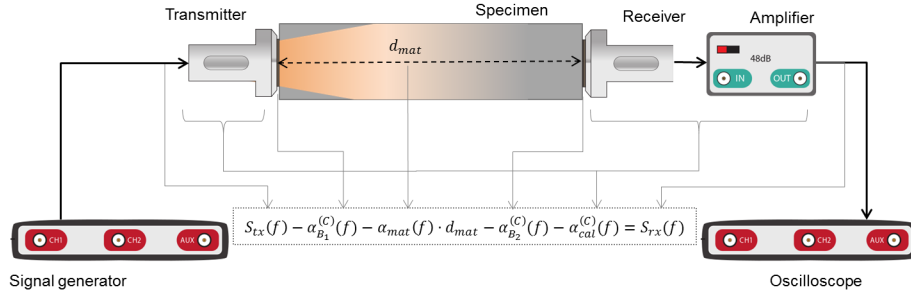
Figure 1: Layout of the equipment used in a contact inspection. The terms of Eq. 3 are identified in each stage of the scheme
