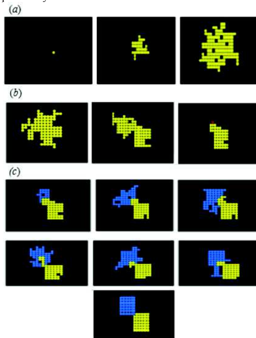
Figure 2. Development of a target shape from a single cell.
