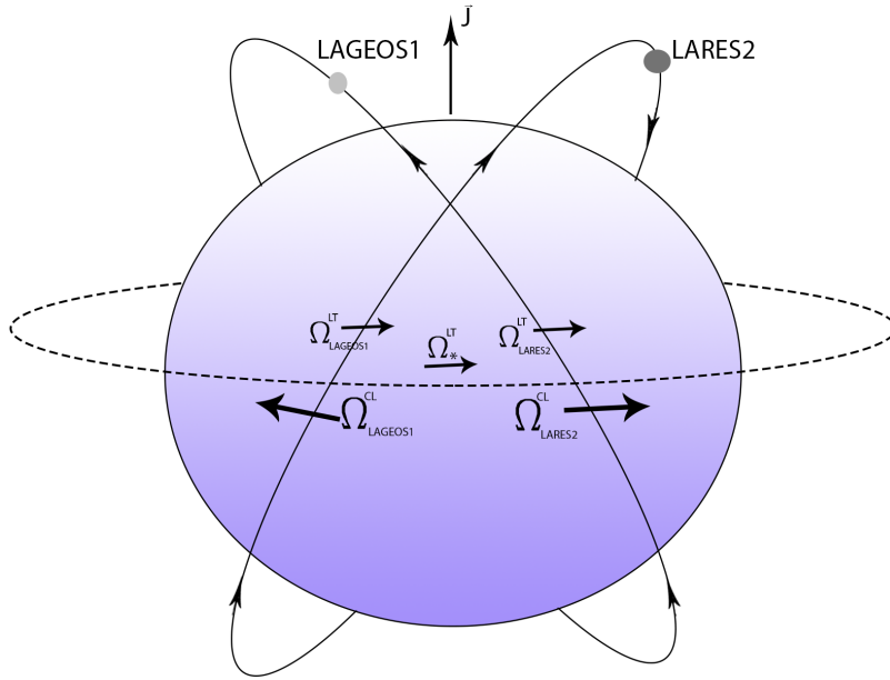
Figure 1. The idea of the LARES 2 experiment (originally called LAGEOS 3) [24,25] In the figure we show frame-dragging and the Newtonian precession of the nodes of two satellites with supplementary inclinations such as LARES 2 and LAGEOS (Supplementary inclinations: i_1 + i_2 = 180^\circ ).
