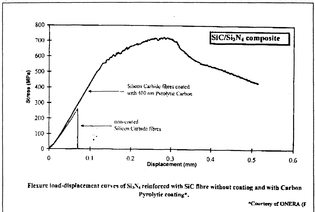
Fig. 1 - Stress-displacement curves
