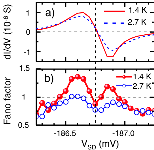
FIG. 4 (color online). (a) Differential conductance for a peak in the I - V characteristic at T \approx 1.4 K and T \approx 2.7 K. (b) The filled symbols show the Fano Factor \alpha at T \approx 1.4 K and the open circles show \alpha at T \approx 2.7 K.
