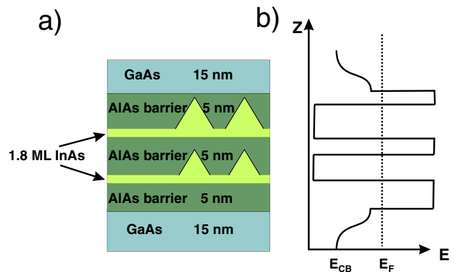
FIG. 1 (color online). (a) Growth scheme of the active part of the device. (b) Conduction band structure E_{CB} and the Fermi energy E_F of a stack of two QDs. If a positive bias voltage is applied the electrons tunnel in positive z direction through the device.
