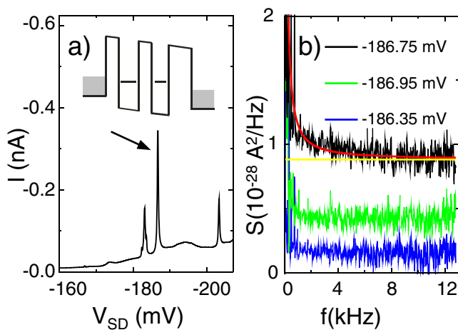
FIG. 2 (color online). (a) Current-voltage characteristics of the sample at T \approx 1.4 K. The arrow marks the peak which is discussed further. Inset: Schematic band structure of the coupled quantum dots where resonant tunneling is observed. (b) Typical noise spectra of the sample for different bias voltages. The solid line demonstrates the results of fitting the function A/f + S_0 to the spectrum at V_{\text{SD}} = -186.75 mV. The horizontal line shows S_0 .
