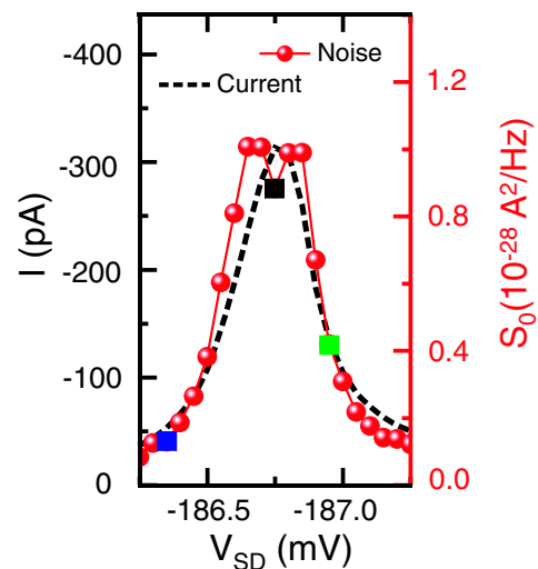
FIG. 3 (color online). Blow up of the peak marked in Fig. 2 in the current-voltage characteristic measured at T \approx 1.4 K (dashed line, left axis) and shot noise amplitude S_0 as given by fitting the function A/f + S_0 to the noise spectra shown in Fig. 2 (dots, right axis). The squares correspond to the spectra shown in Fig. 2(b). The scale of the right axis was chosen such that the dashed line corresponds on this axis to full shot noise S_{\text{full}} = 2eI as expected for a single tunneling barrier structure (Fano factor \alpha = 1 ).
