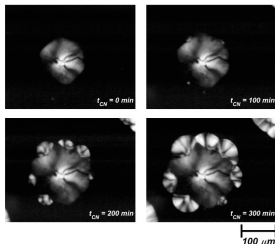
Figure 2. Optical micrographs taken at different times ( t_{CN} , indicated) during a cross-nucleation experiment at 145 °C. The more birefringent \alpha -phase spherulites nucleate at the advancing front of a \beta -hedrite initially grown at 139 °C.
