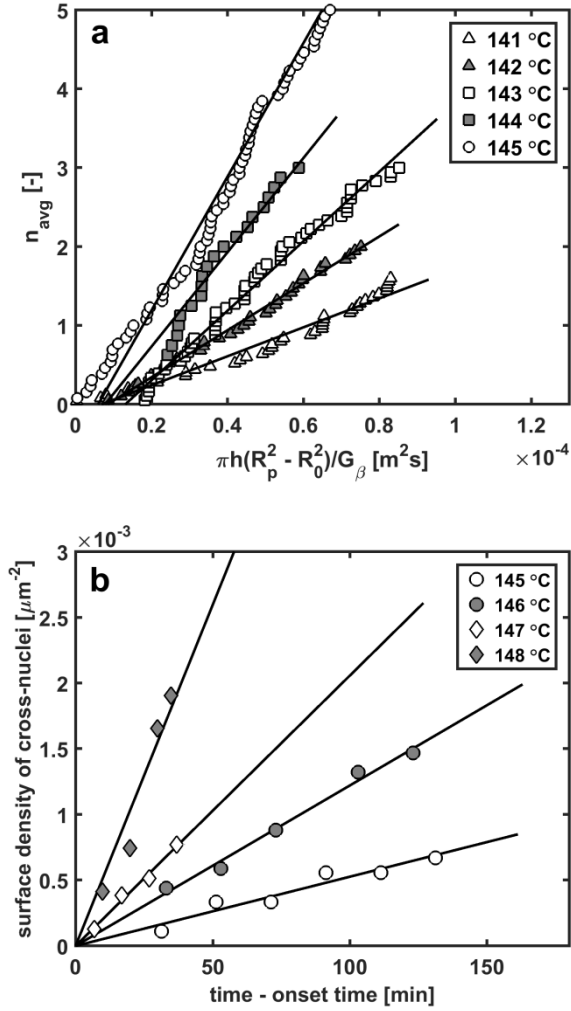
Figure 5. a) Average number of \alpha -cross-nuclei as a function of the “normalized” ( R_{p,i}^2 - R_{o,i}^2 ) (according to Equation S2 and S3 of the Supporting Information). Results relative to different indicated cross-nucleation temperatures are shown; b) Number of \alpha -phase cross-nuclei per unit area of \beta -hedrite lateral surface as a function of time, at the indicated cross-nucleation temperatures. In both plots, the slope of the fitted lines represents the cross-nucleation rate.
