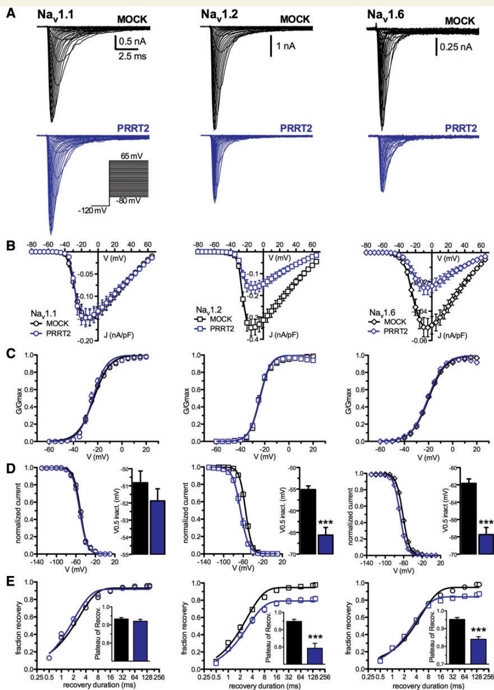
Figure 6 PRRT2 expression decreases the Na^+ current density of Na_v1.2 and Na_v1.6 , but not of Na_v1.1 , expressed in HEK-293 cells. (A) Representative whole-cell currents recordings on clones stably expressing Na_v1.1 (left), Na_v1.2 (middle) and Na_v1.6 (right) and transiently transfected with empty vector (MOCK, black) or PRRT2 (blue). Currents were evoked by 5-mV steps depolarization from -80 to 65 mV and cells were held at -120 mV (inset). (B) Current density versus voltage relationship for the genotypes described in A . (C) Voltage-dependence of activation for the three Na_v channels co-expressed with MOCK or PRRT2. The lines are the best-fitted Boltzmann curves with the following mean values of half maximal voltage activation ( V_{0.5} ) and slope ( k ): Na_v1.1 , MOCK, V_{0.5} : -23.12 \pm 0.27 mV, k : 6.58 \pm 0.23 ( n = 38 ), PRRT2 V_{0.5} : -24.00 \pm 0.24 , k : 5.67 \pm 0.21 ( n = 34 ); Na_v1.2 , MOCK, V_{0.5} : -23.89 \pm 0.19 mV, k : 4.39 \pm 0.16 ( n = 22 ), PRRT2 V_{0.5} : -24.16 \pm 0.21 ; k : 4.37 \pm 0.19 ( n = 20 ); Na_v1.6 , MOCK, V_{0.5} : -19.81 \pm 0.14 mV, k : 6.99 \pm 0.12 ( n = 27 ), PRRT2 V_{0.5} : -20.46 \pm 0.17 , k : 6.83 \pm 0.15 ( n = 29 ). (D) Steady-state inactivation curves for all conditions tested. The lines are the best-fitted Boltzmann curves and the half-maximal voltages for inactivation ( V_{0.5} inact.) was graphed on the right. Data are means \pm SEM ( Na_v1.1 : MOCK, n = 36 and PRRT2; n = 30 ; Na_v1.2 : MOCK, n = 22 and PRRT2, n = 18 ; Na_v1.6 : MOCK, n = 24 and PRRT2, n = 21 ). (E) Time-dependent rate of recovery from inactivation. The plateau values (insets) were estimated from one-phase decay fit to the data. Data are means \pm SEM ( Na_v1.1 : MOCK, n = 33 and PRRT2; n = 24 ; Na_v1.2 : MOCK, n = 21 and PRRT2, n = 18 ; Na_v1.6 : MOCK, n = 20 and PRRT2, n = 18 ). In D and E : *** P < 0.001 ; unpaired Student's t -test or Mann-Whitney U-test.
