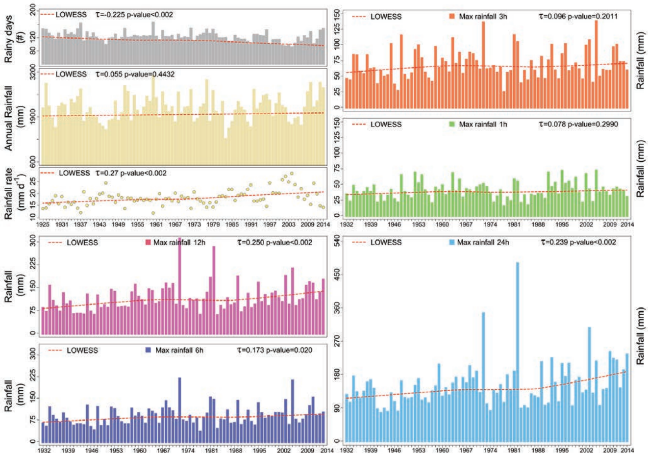
Fig. 9 - Climate series of annual rainfall, rainy days and rainfall rate in Diga Giacopiane weather station from 1925 to 2014 (top left). Maximum annual rainfall for 1, 3, 6, 12 and 24 h at Diga di Giacopiane rain gauge from 1932 to 2014)
